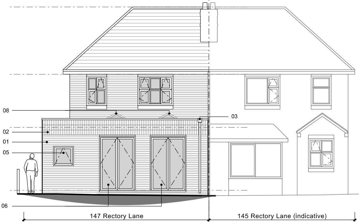
Rear Elevation (North)
