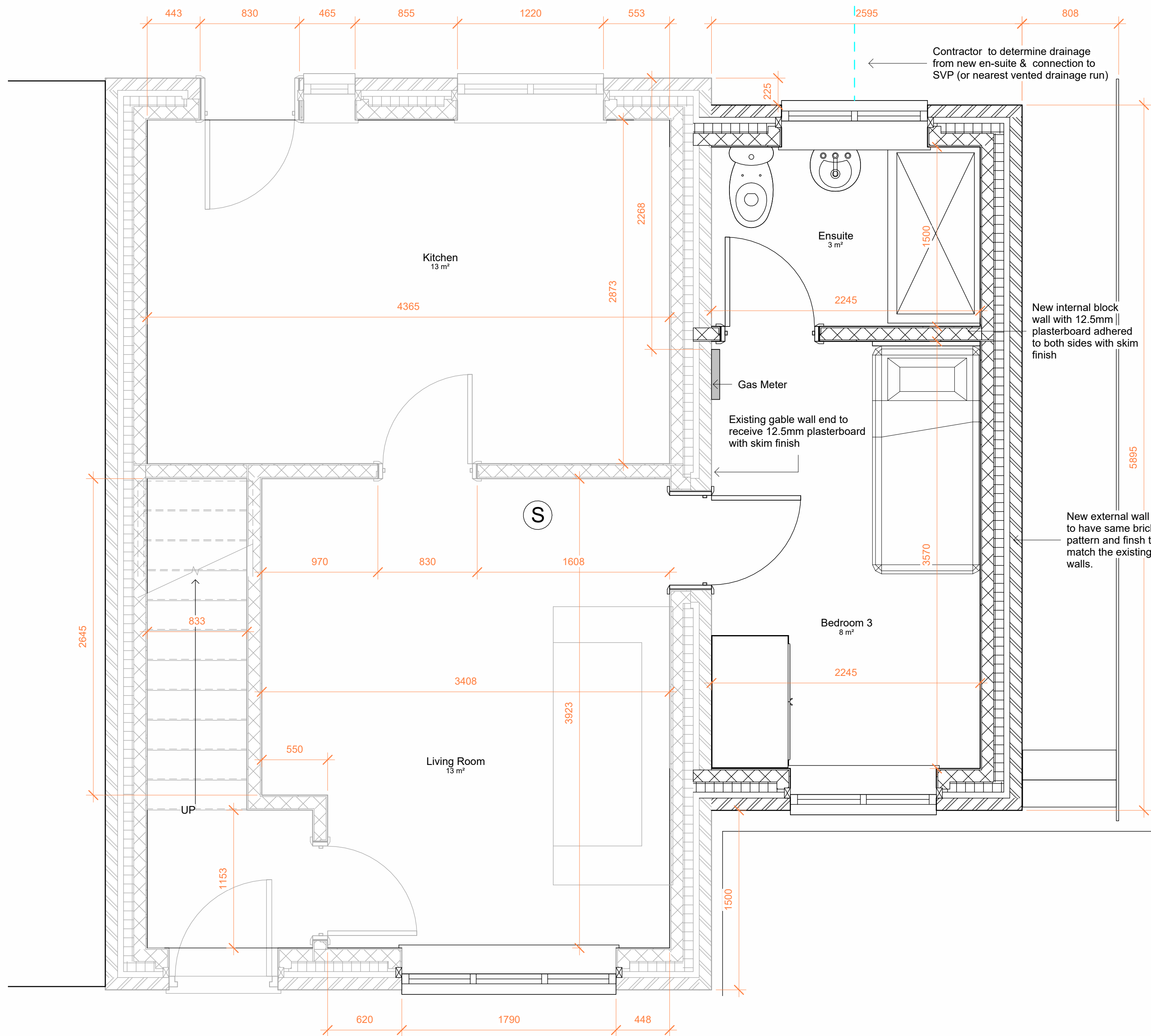
Ground Floor 1 : 25
