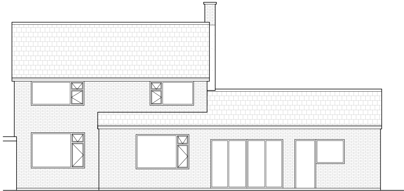
EXISTING REAR ELEVATION 1:100 @ A3
