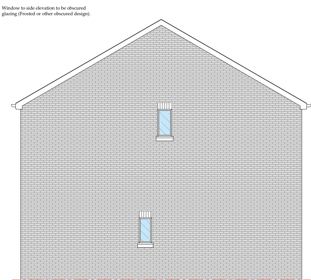
Existing Side Elevation (Scale - 1:75)
