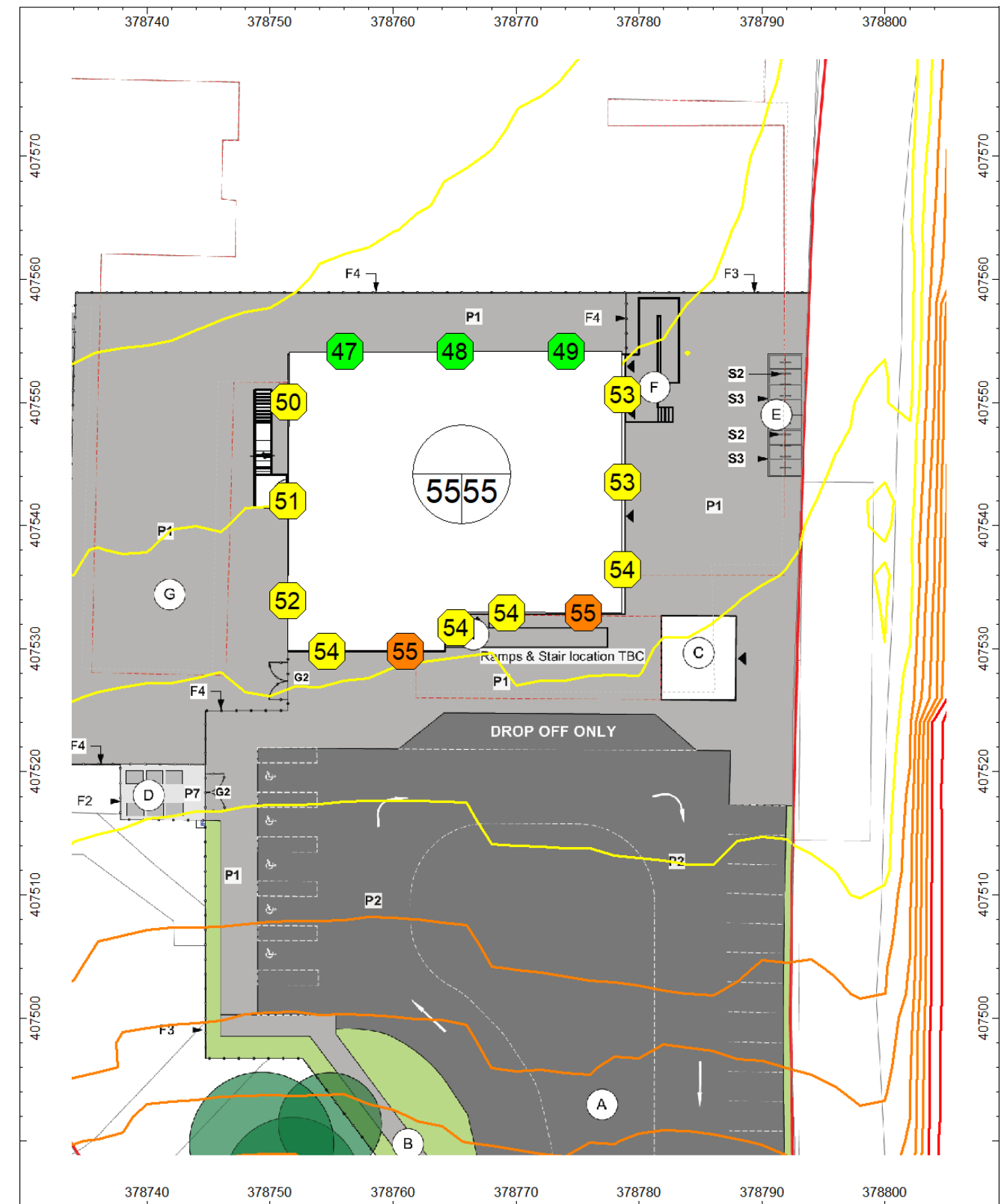
Figure 4: Predicted daytime free-field ambient noise levels on the façades of the Temporary block, dB L_{Aeq,30min}
