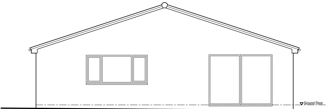
REAR ELEVATION AS EXISTING
