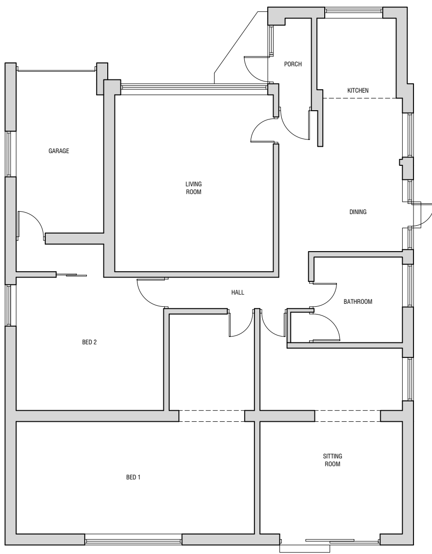
FLOOR PLAN AS EXISTING
