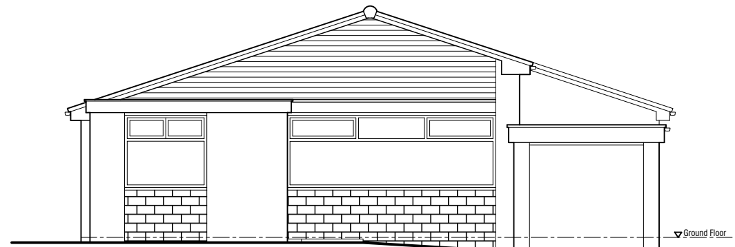
FRONT ELEVATION AS EXISTING
