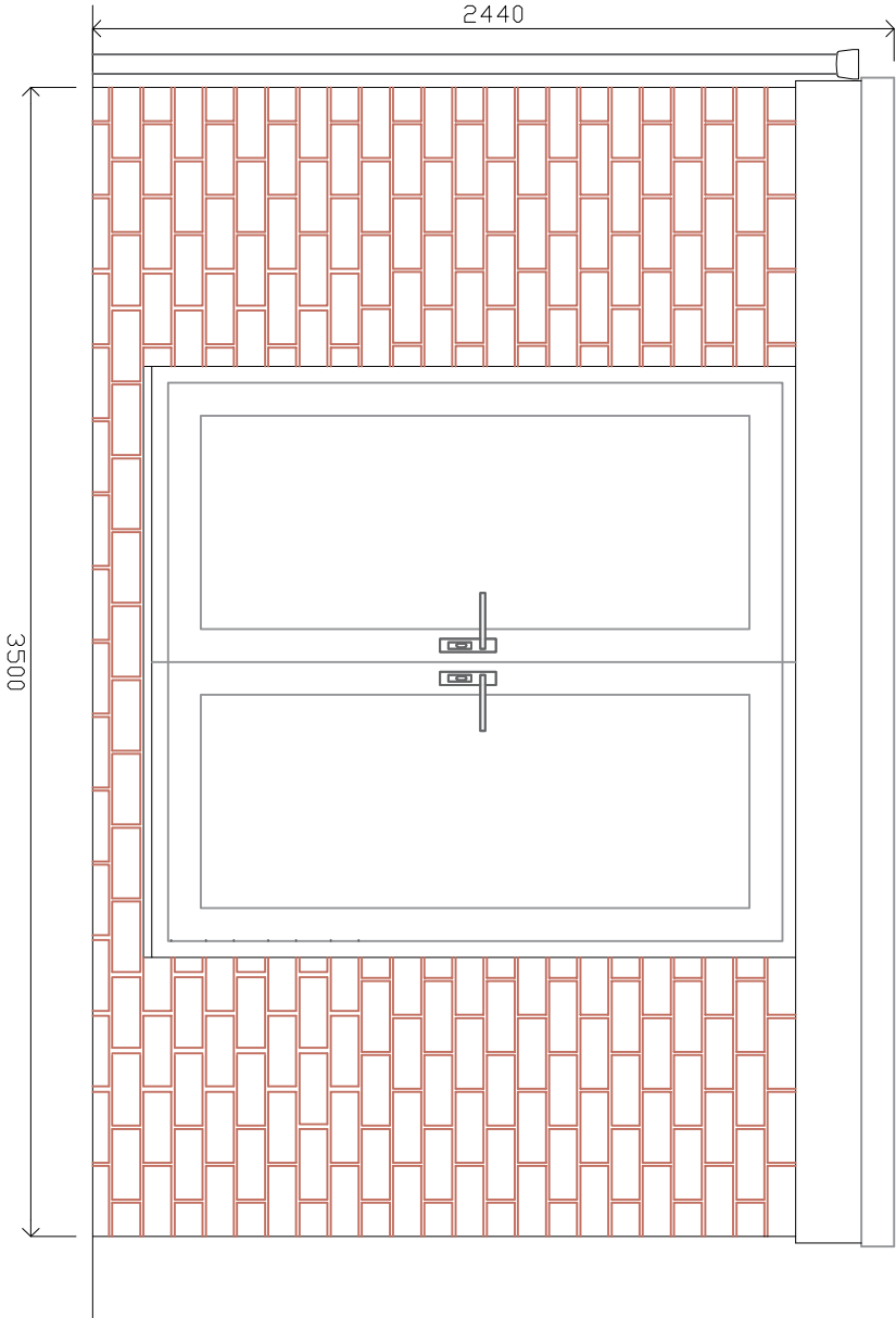
Proposed Rear:
