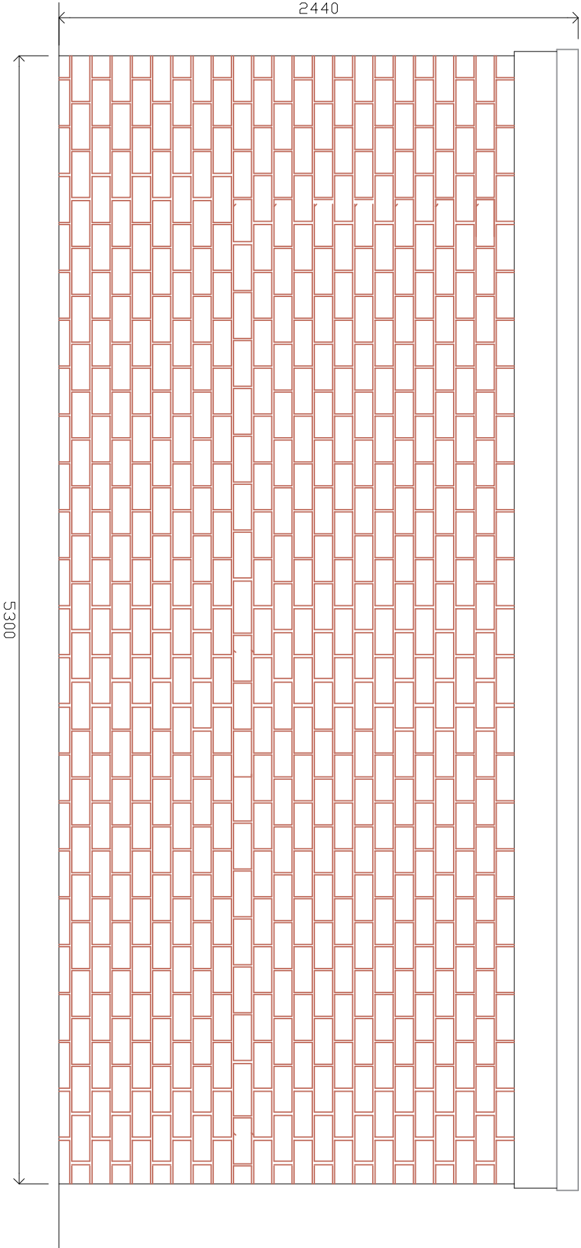
Existing Side 1:
