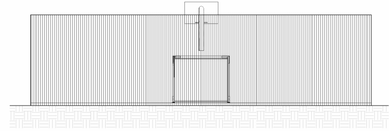
4 MUGA - East 1:50
