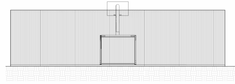
2 MUGA - West 1:50
