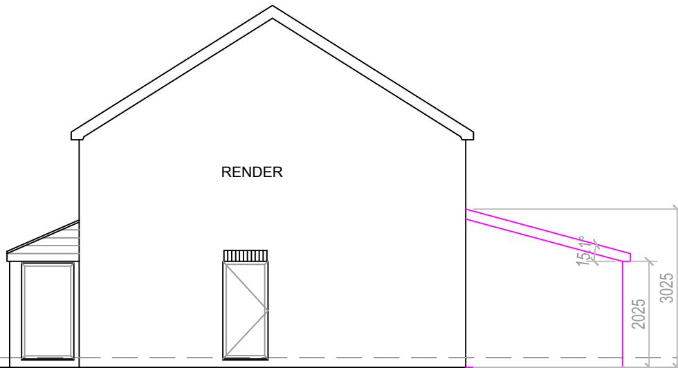
PROPOSED GABLE ELEVATION
