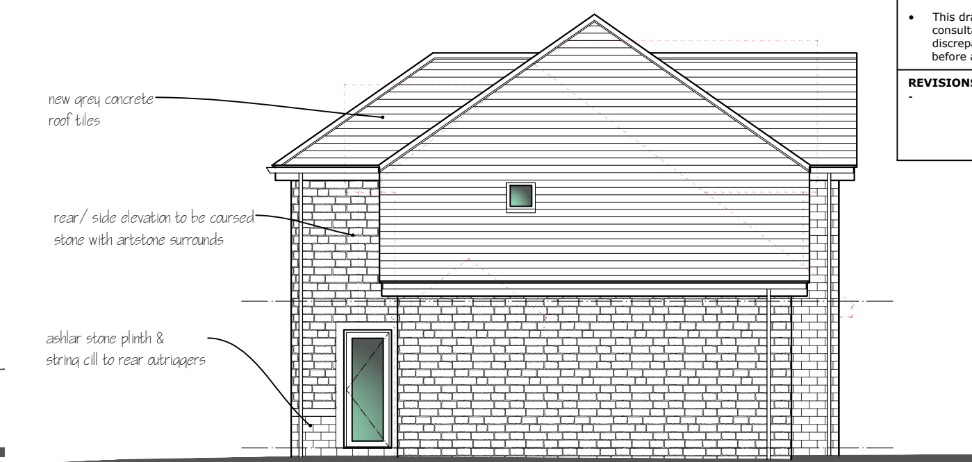
SIDE ELEVATION (facing 4 Windrush Ave.)
