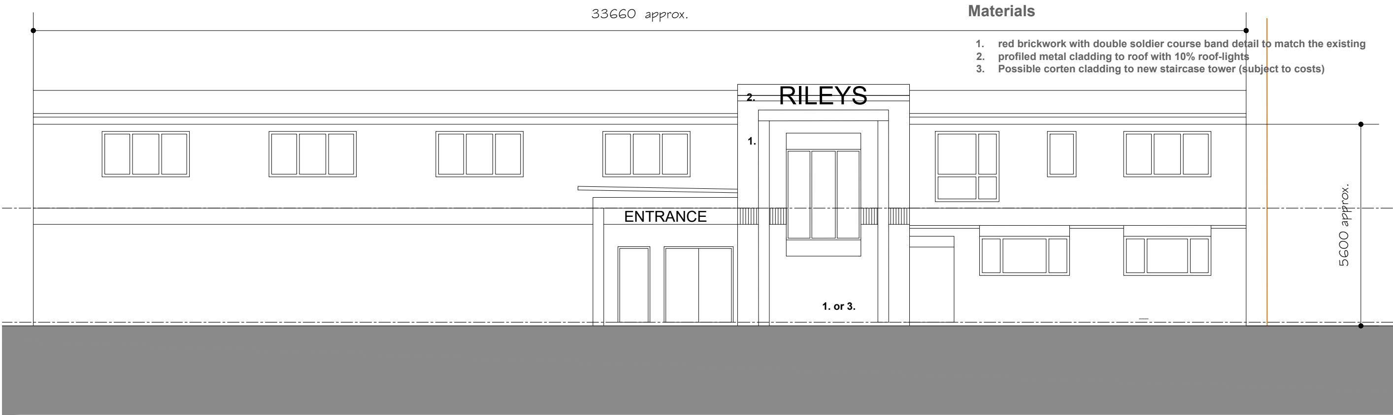
front elevation
