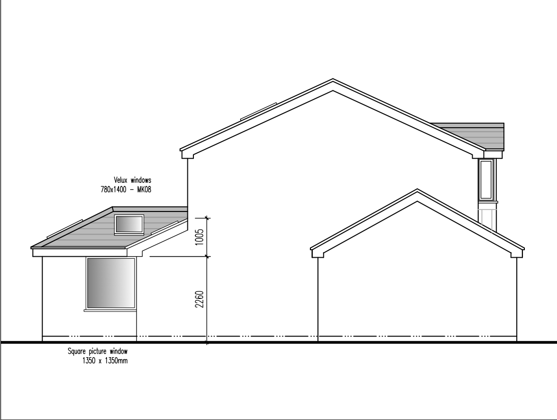
ELEVATION - SIDE 2
