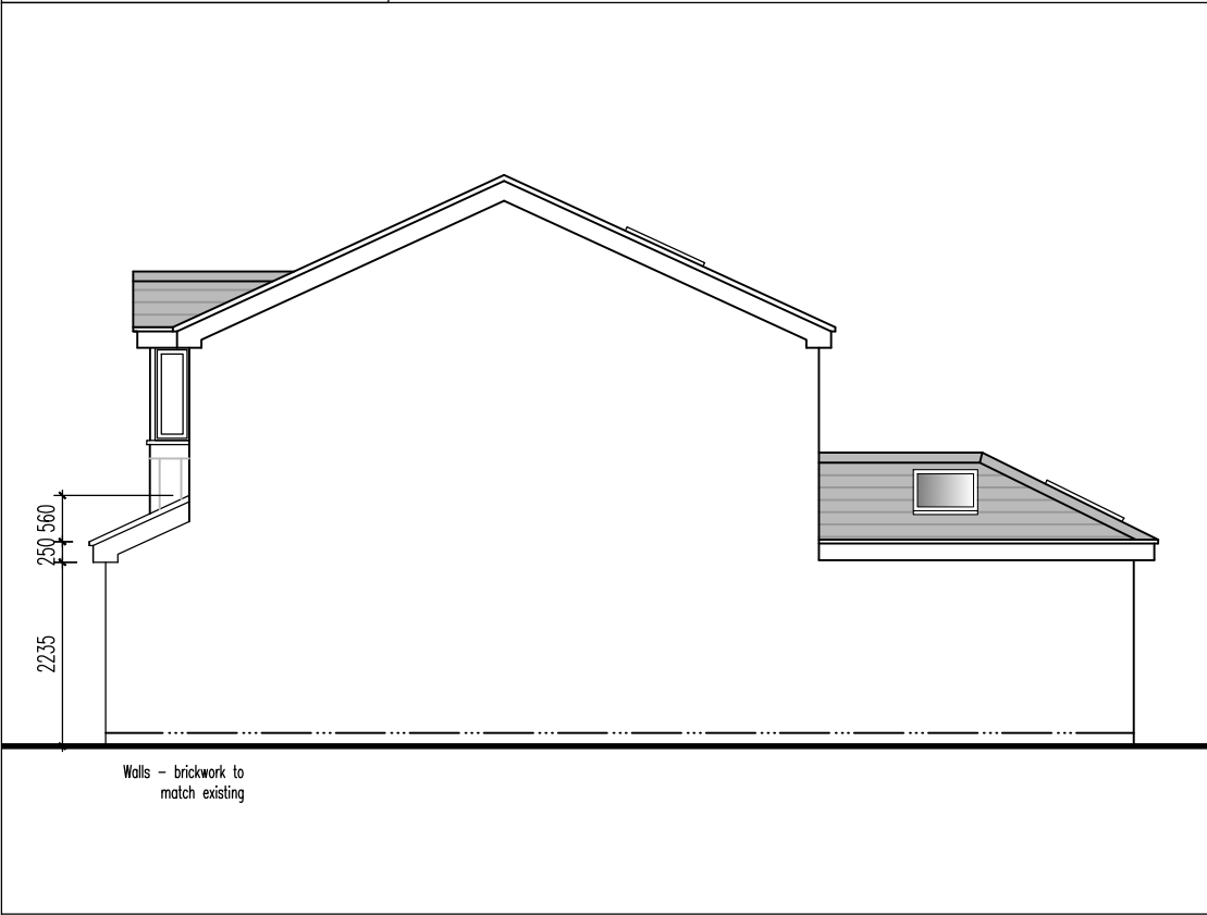
ELEVATION - SIDE 1
