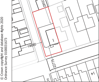
LOCATION PLAN (1:1250)
