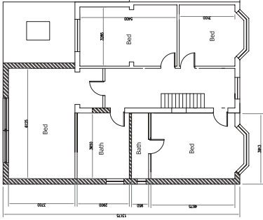
PROPOSED FIRST FLOOR
