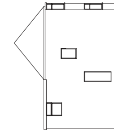
EXISTING SIDE ELEVATION (1)
