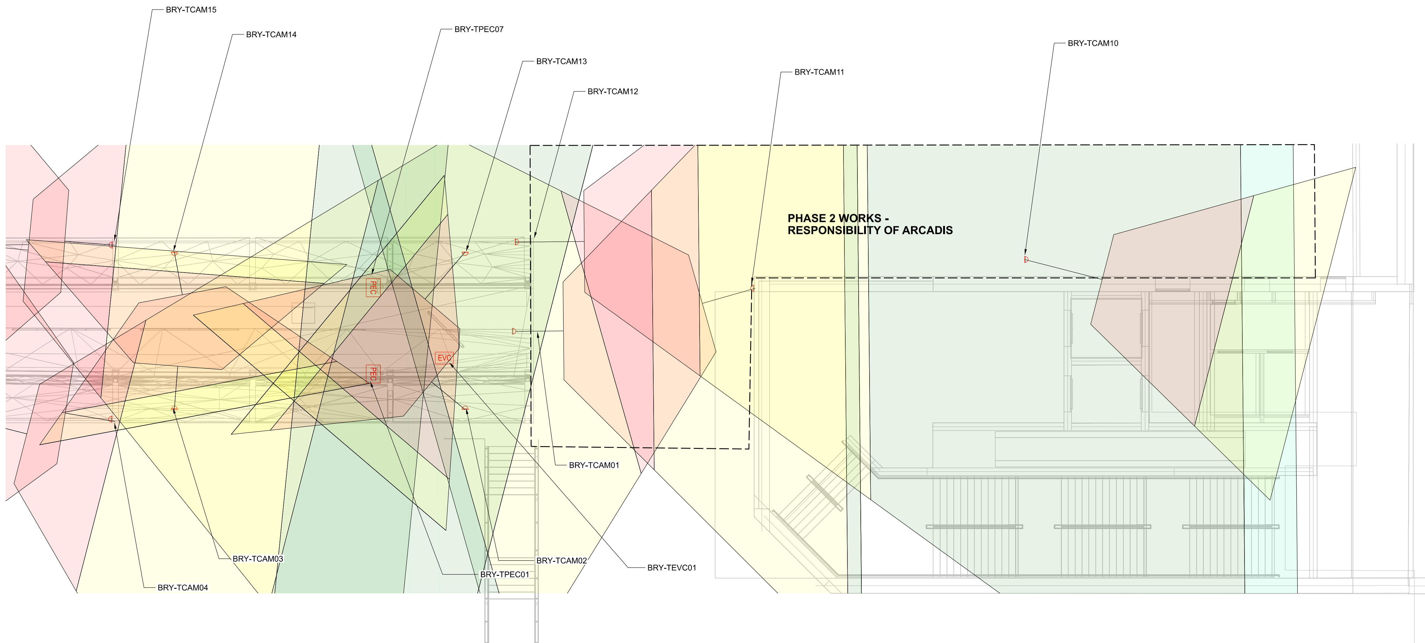
PROPOSED PLATFORM TELECOMS CCTV COVERAGE (1/3) Scale 1:100
