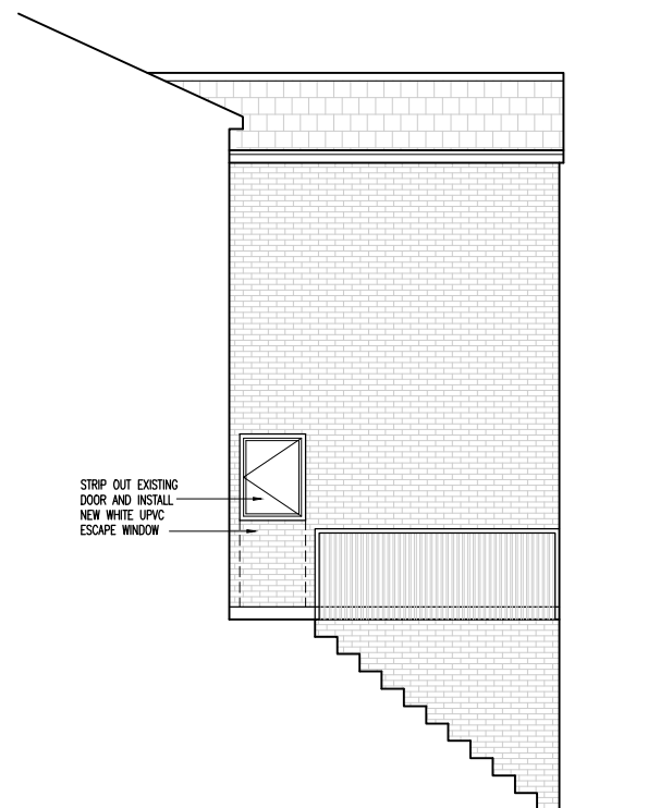
PROPOSED REAR/SIDE ELEVATION 1:100 @ A3
