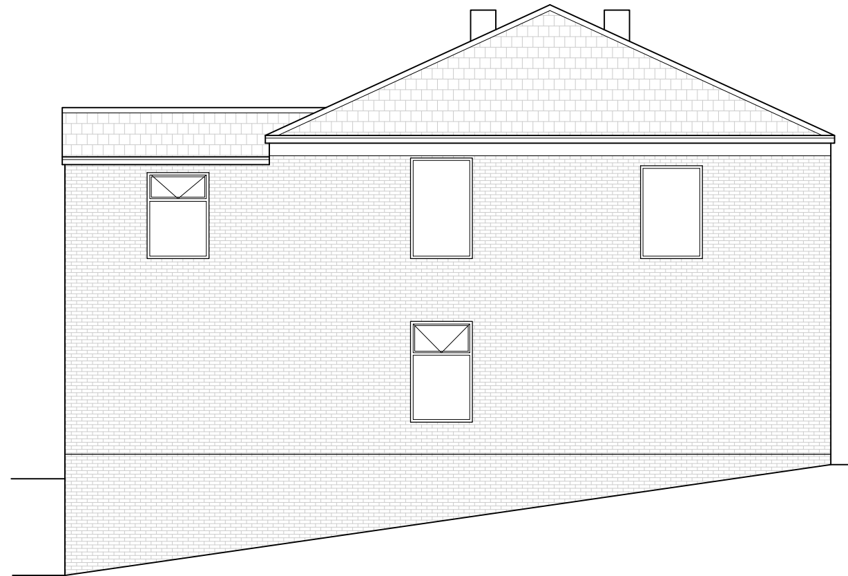
PROPOSED SIDE ELEVATION 1:100 @ A3
