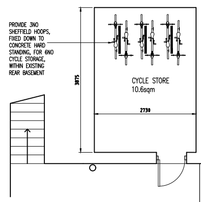
PROPOSED BASEMENT FLOOR PLAN 1:100 @ A3
