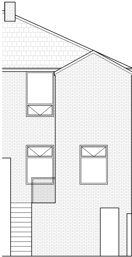
EXISTING REAR ELEVATION 1:100 @ A3
