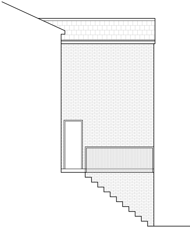
EXISTING REAR/SIDE ELEVATION 1:100 @ A3
