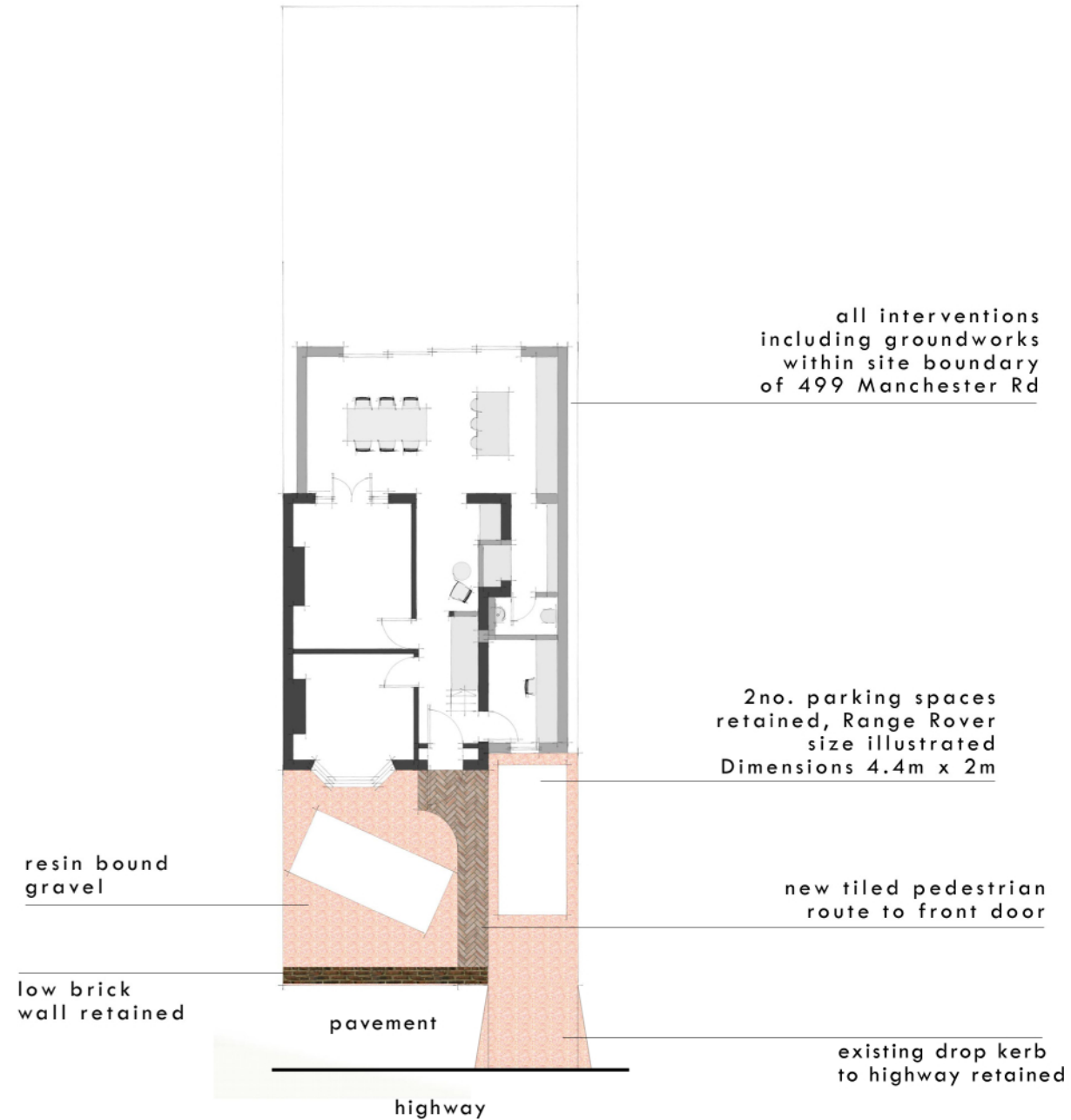
proposed parking layout scale 1:200
