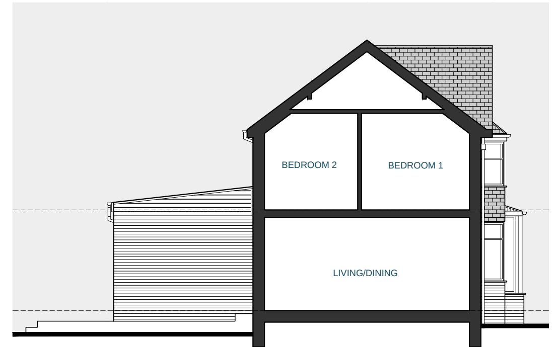
6. North Elevation
