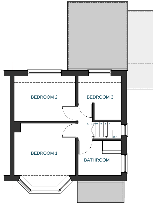
2. First Floor Plan
