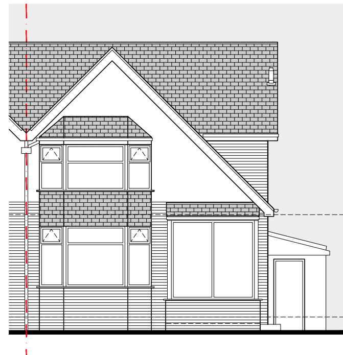
3. West Elevation
