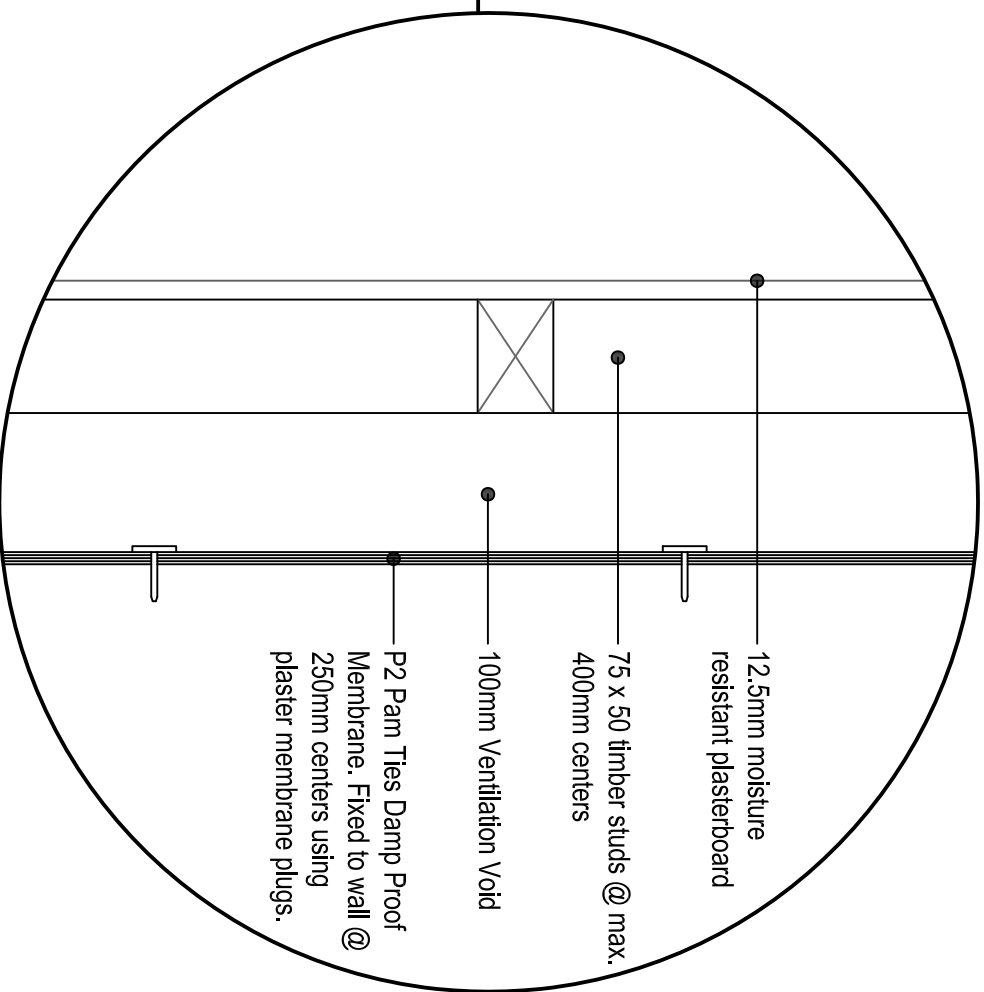
DETAIL 1:5
