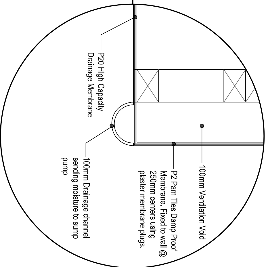
DETAIL 1:5
