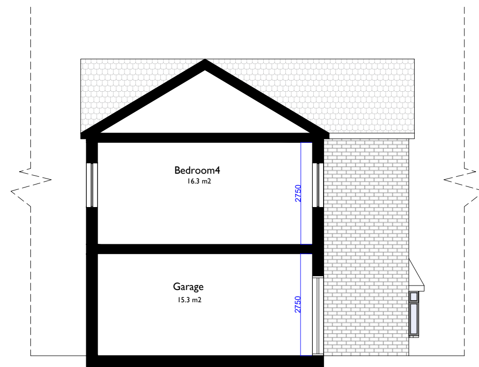
Existing AA Section
