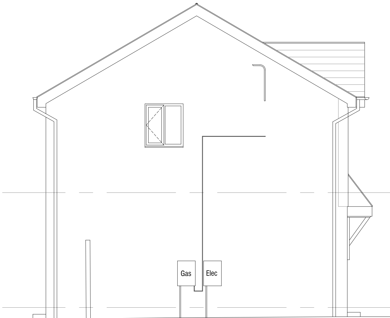
SIDE ELEVATION
