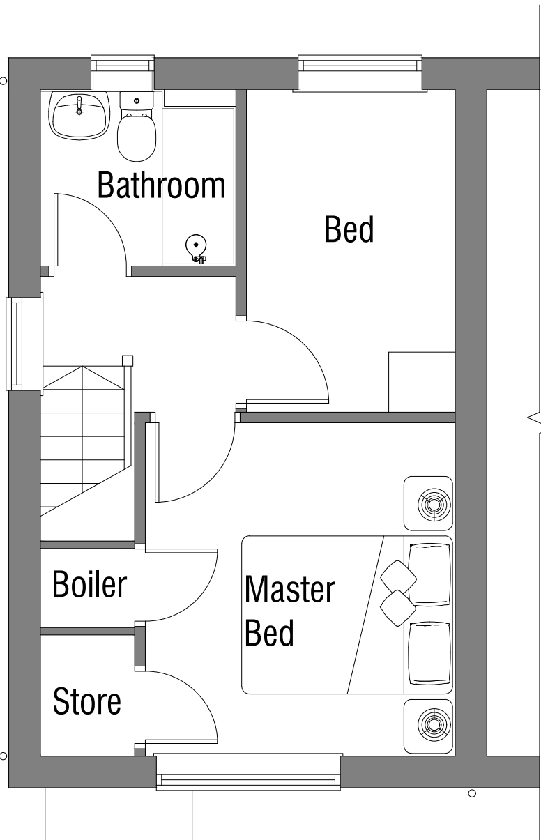
FIRST FLOOR
