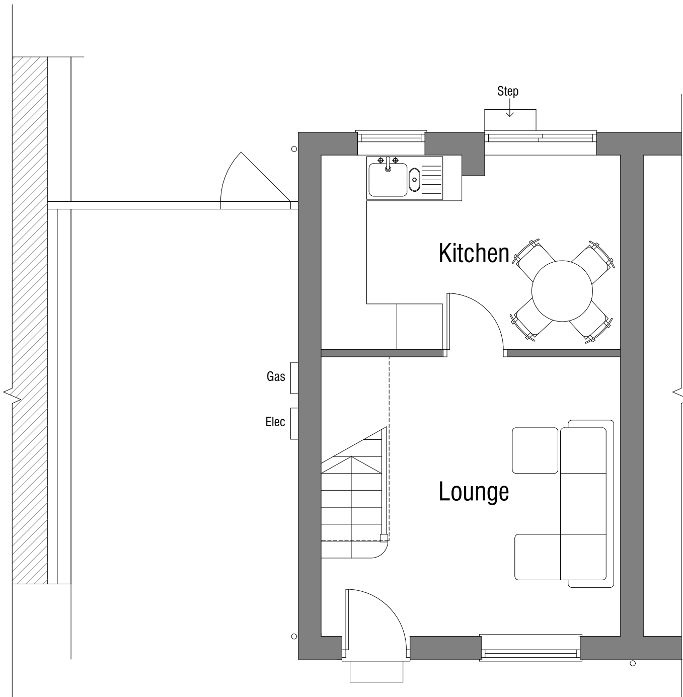
GROUND FLOOR
