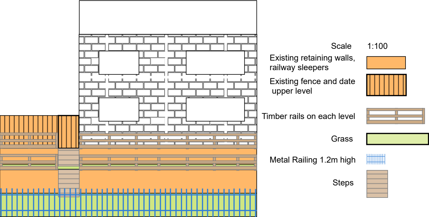
Rear elevation showing existing features only - 19 Ascot Meadow Bury
