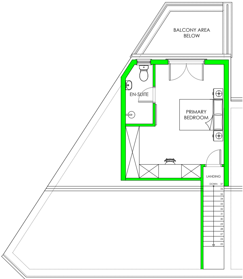
PROPOSED SECOND FLOOR PLAN 1:100
