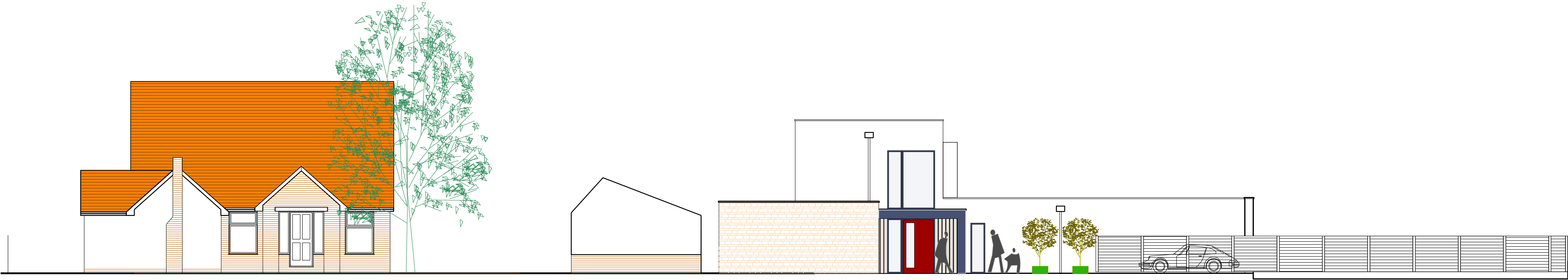
EXISTING WEST STREET SCENE ALONG WOODHEY ROAD 1:100
