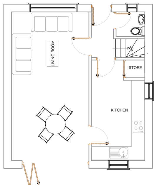
PROPOSED GROUND FLOOR PLAN Internal Gross area 40 sqm
