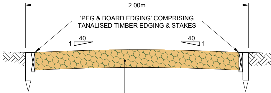
TYPICAL SECTION THROUGH PUBLIC FOOTPATH SCALE - 1:20
