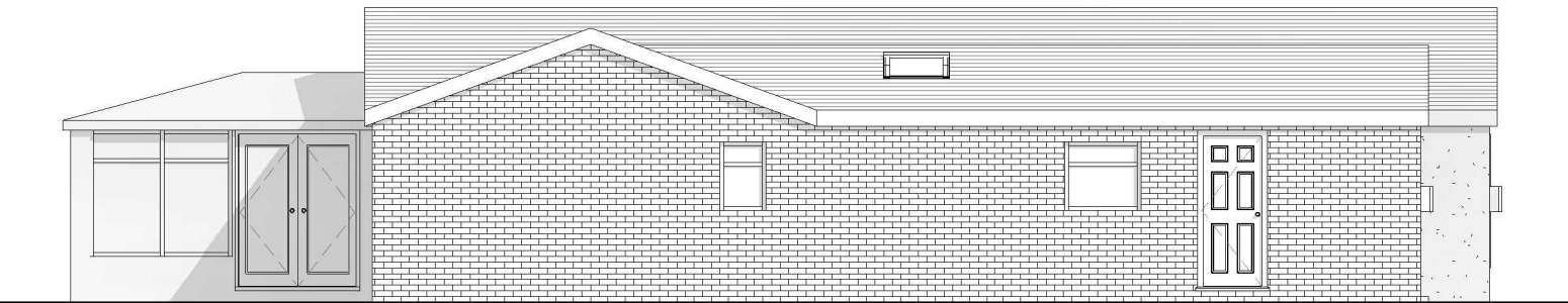
side elevation
