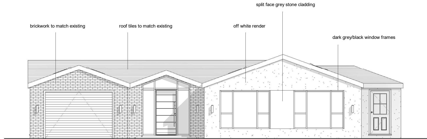
front elevation
