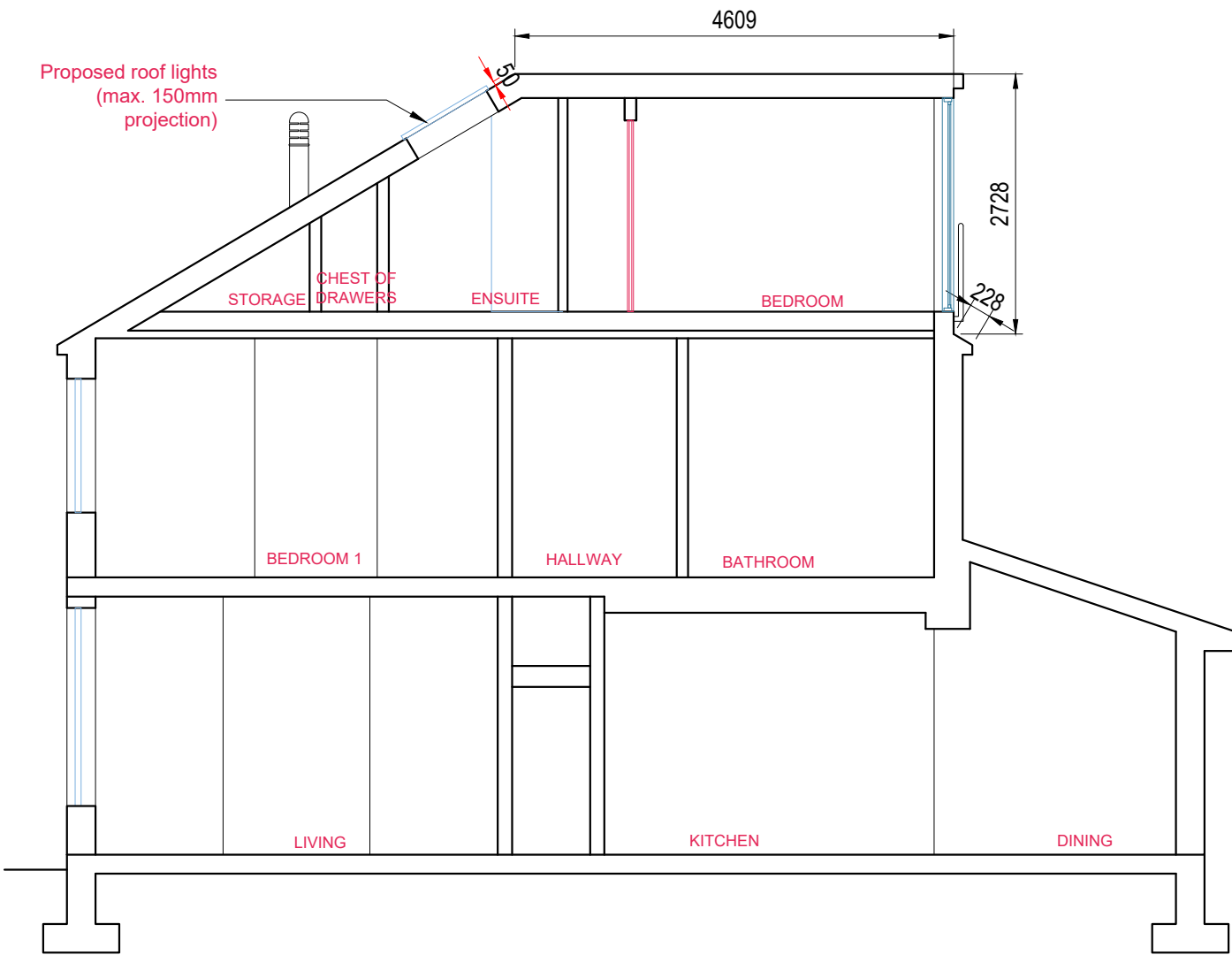
PROPOSED SECTION C-C
