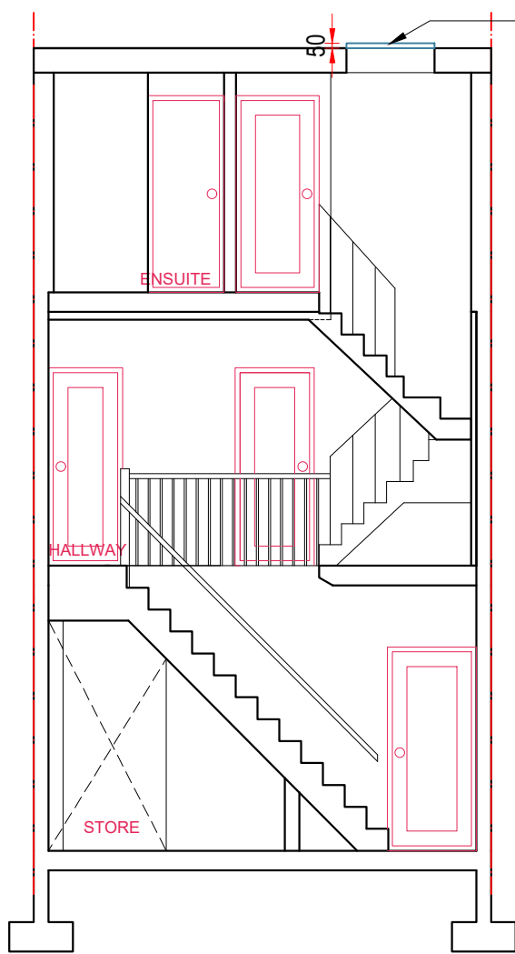
PROPOSED SECTION A-A
