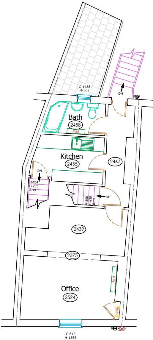
Existing First Floor Plan 1:100
