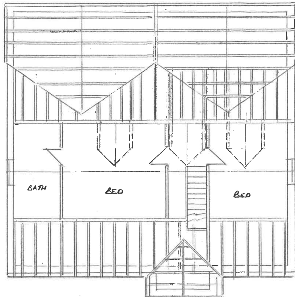
PROPOSED LOFT PLAN
