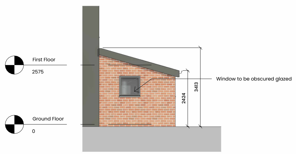
1 Proposed Side Elevation B. 1 : 100
