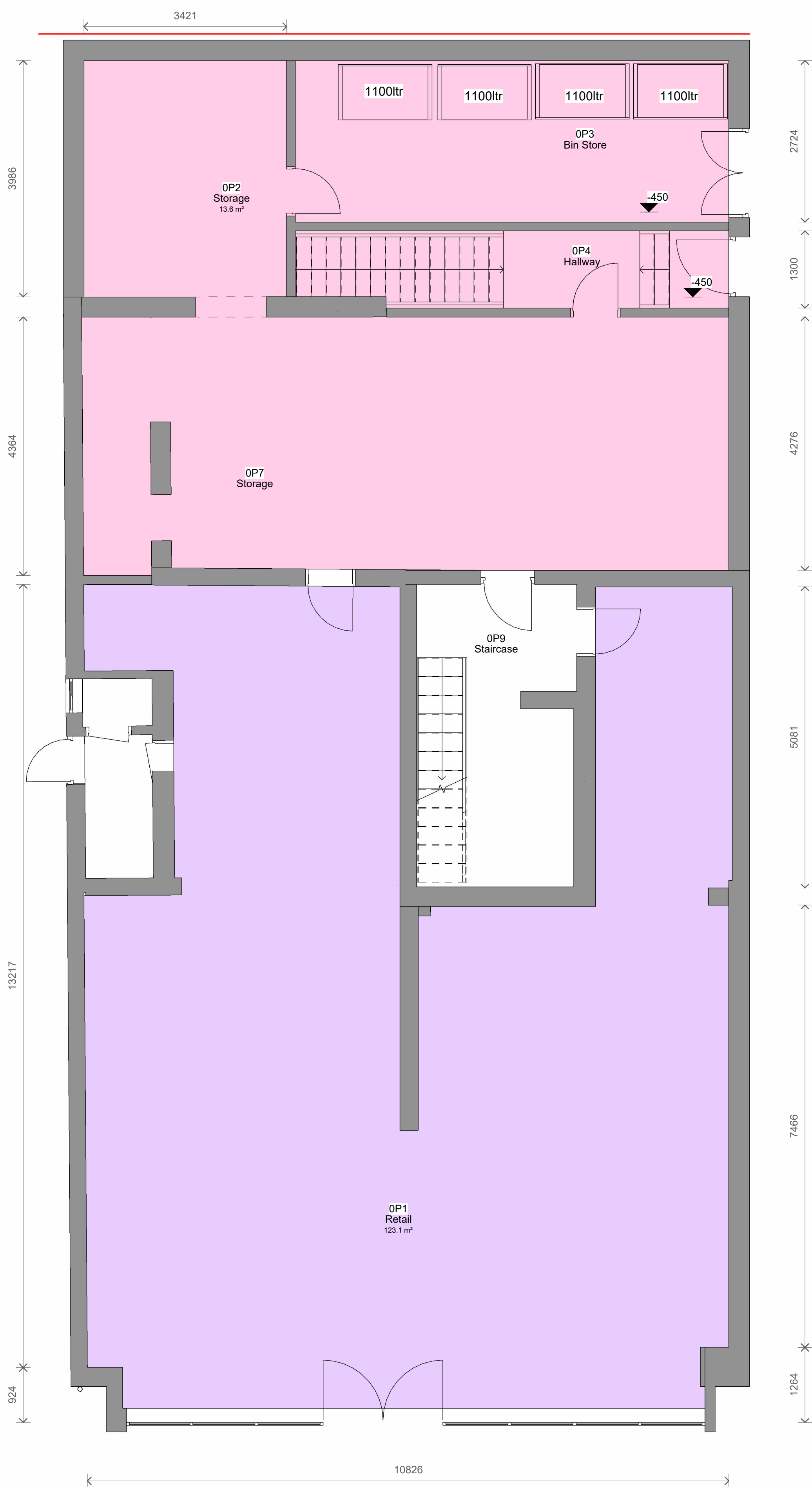
2 Level 0 - Proposed 1 : 50
