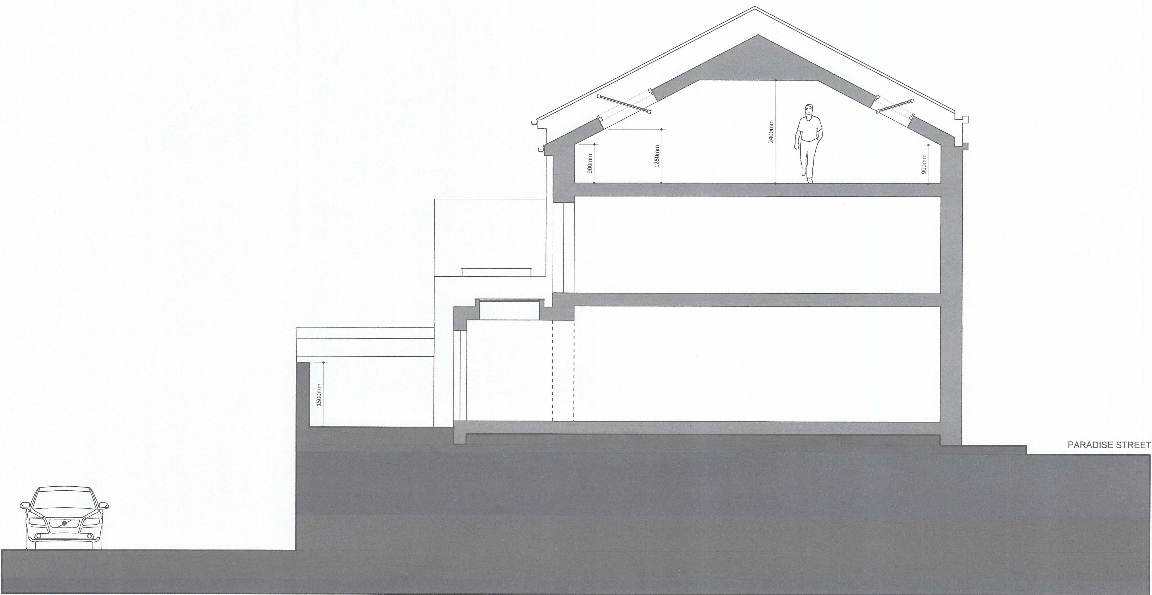
EAST - WEST SECTION THROUGH THE SMITHY/THE FORGE
