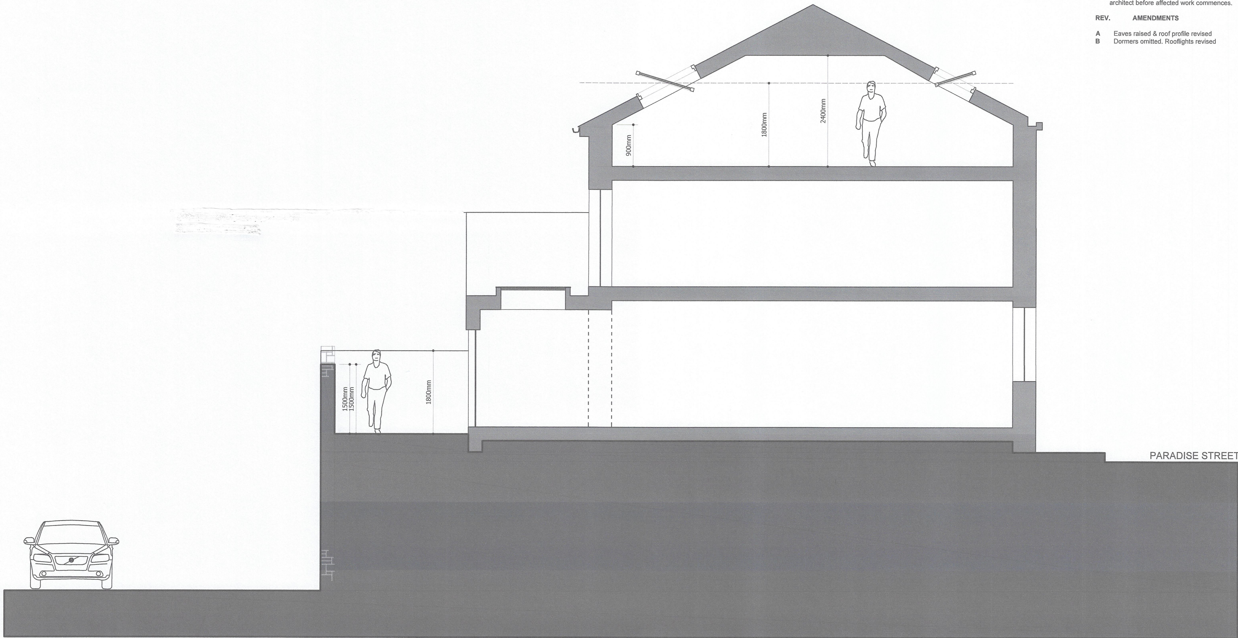
EAST - WEST SECTION THROUGH 12 PARADISE STREET
