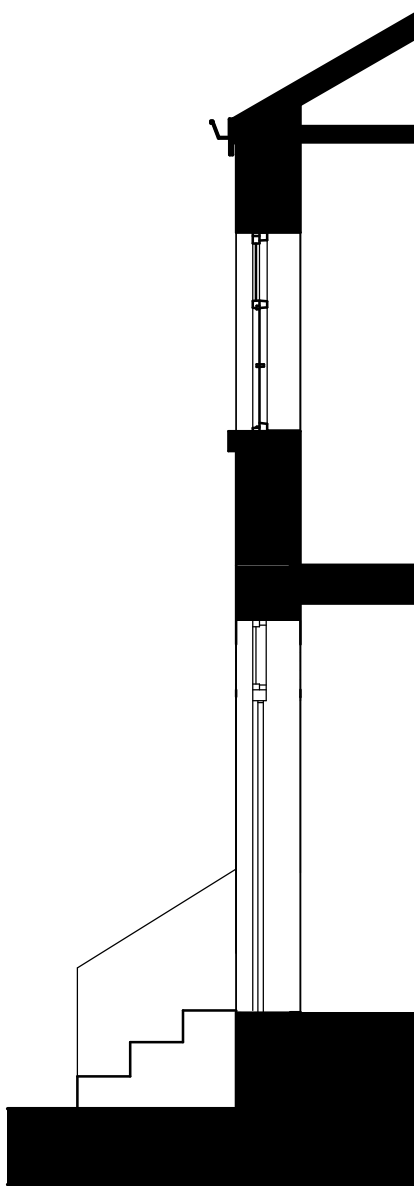
Window 2 Full Section 1 : 50
