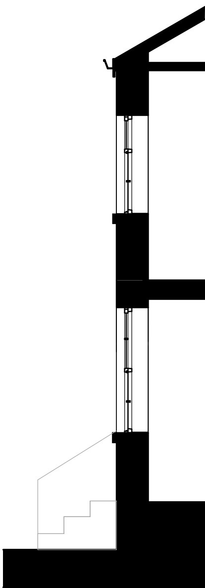
Window 3 Full Section 1 : 50
