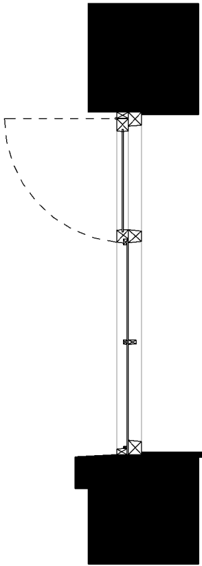
Window 2 Detail Section 1 : 20
