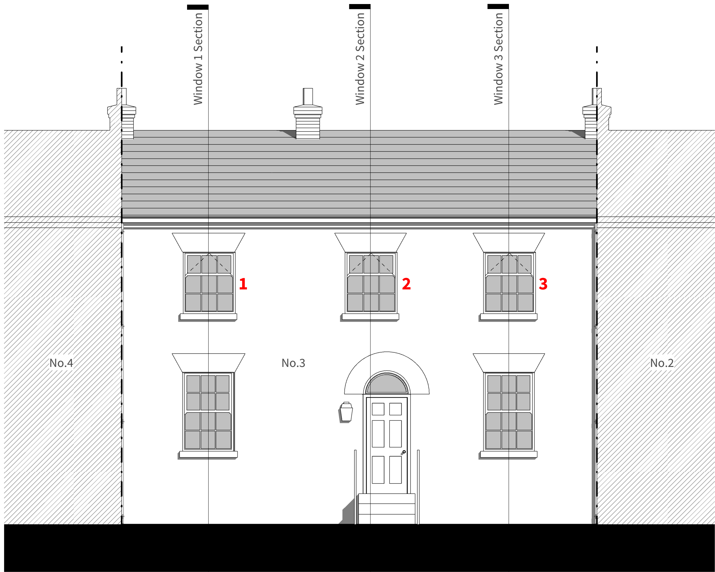
Front Elevation 1 : 50
