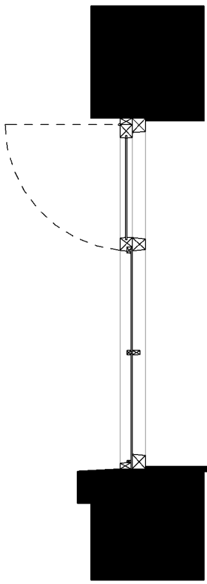
Window 1 Detail Section 1 : 20
