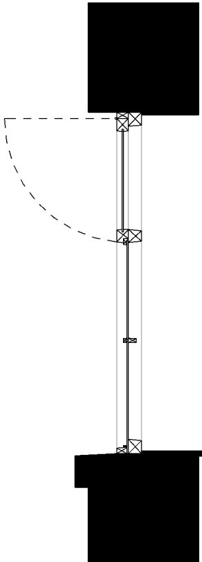
Window 3 Detail Section 1 : 20
