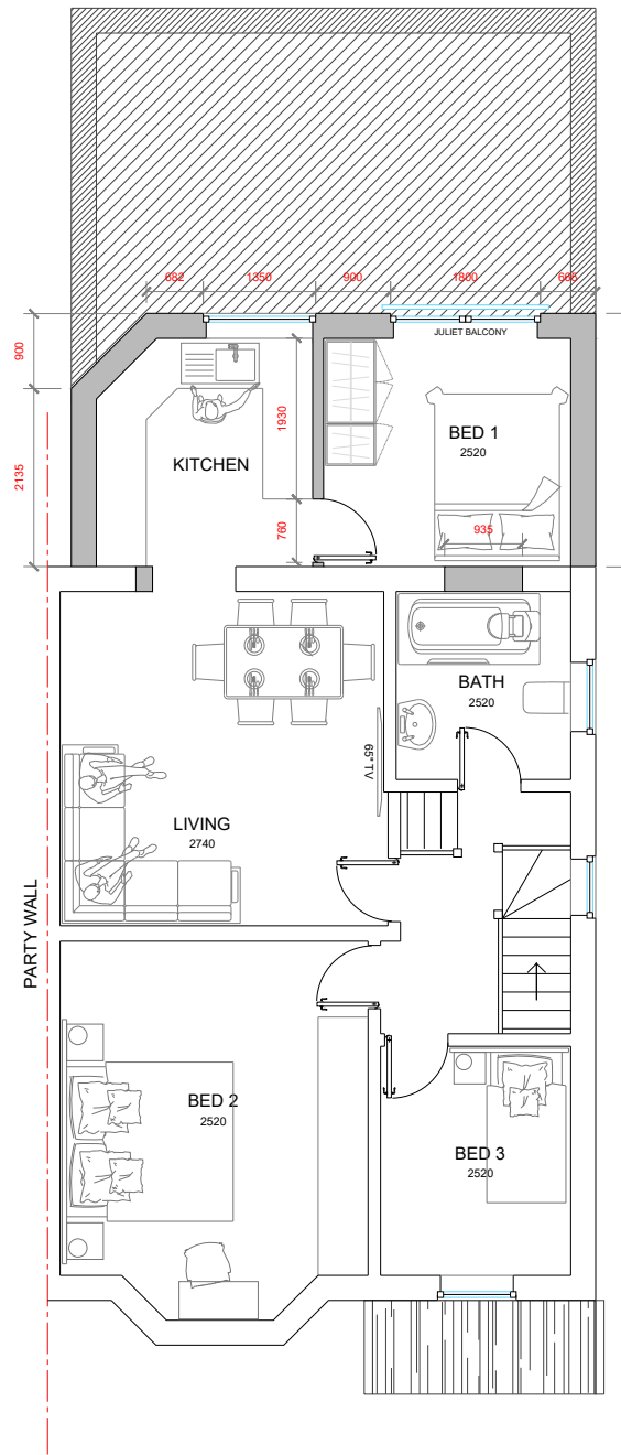
FIRST FLOOR
