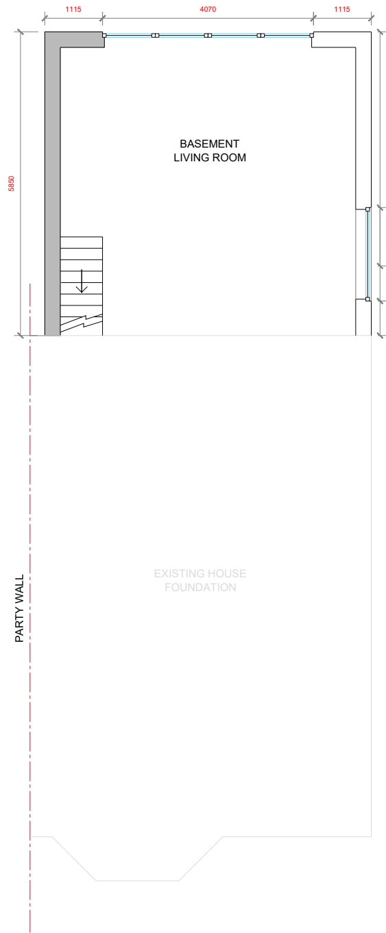
BASEMENT PLAN
