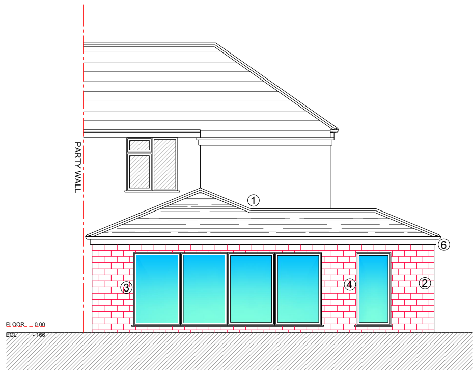
REAR ELEVATION
