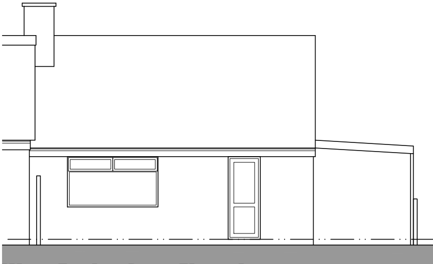
West Facing Rear Elevation
