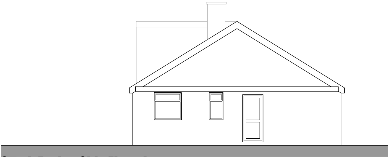
South Facing Side Elevation
