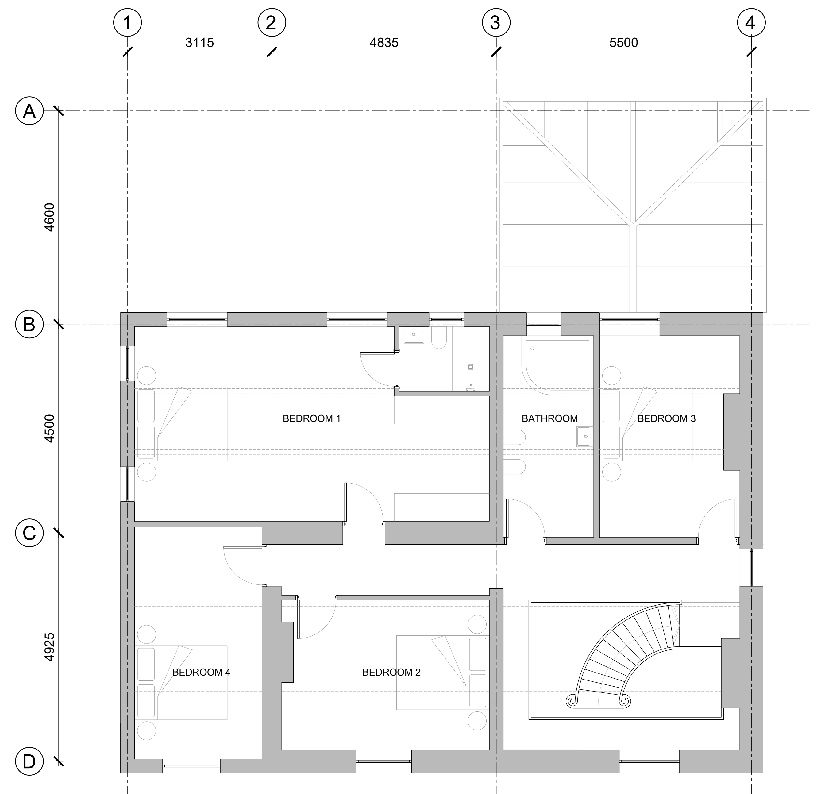
EXISTING FIRST FLOOR
