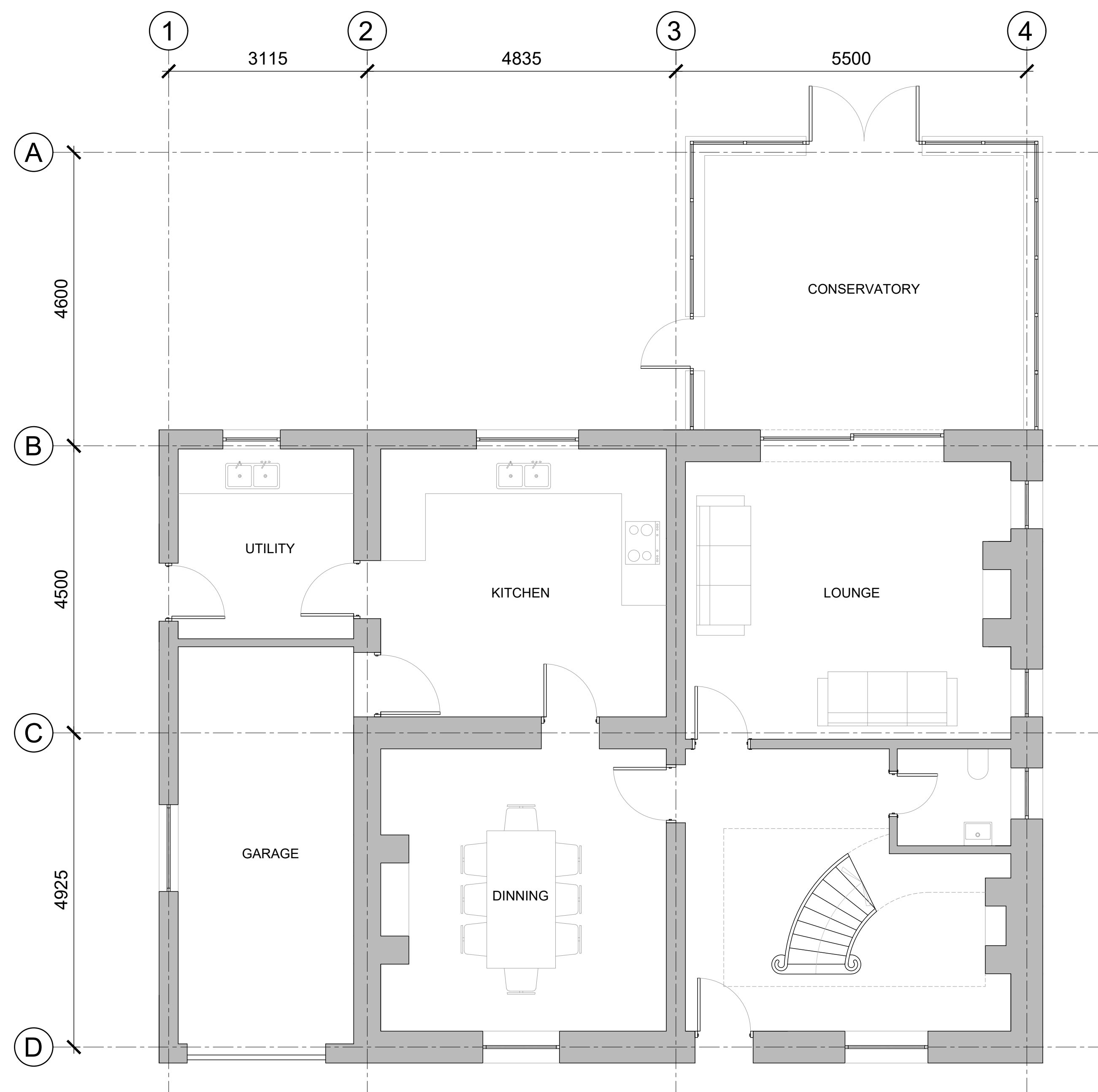
EXISTING GROUND FLOOR
