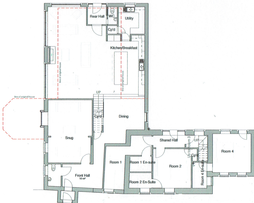
Ground Floor 1 : 100
