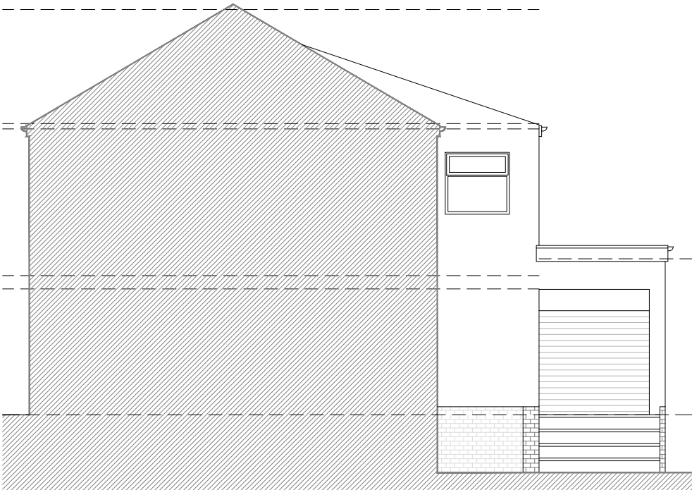
EXISTING GABLE ELEVATION 1:100
