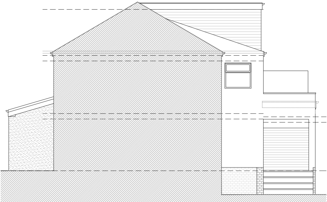
PROPOSED GABLE ELEVATION 1:100
