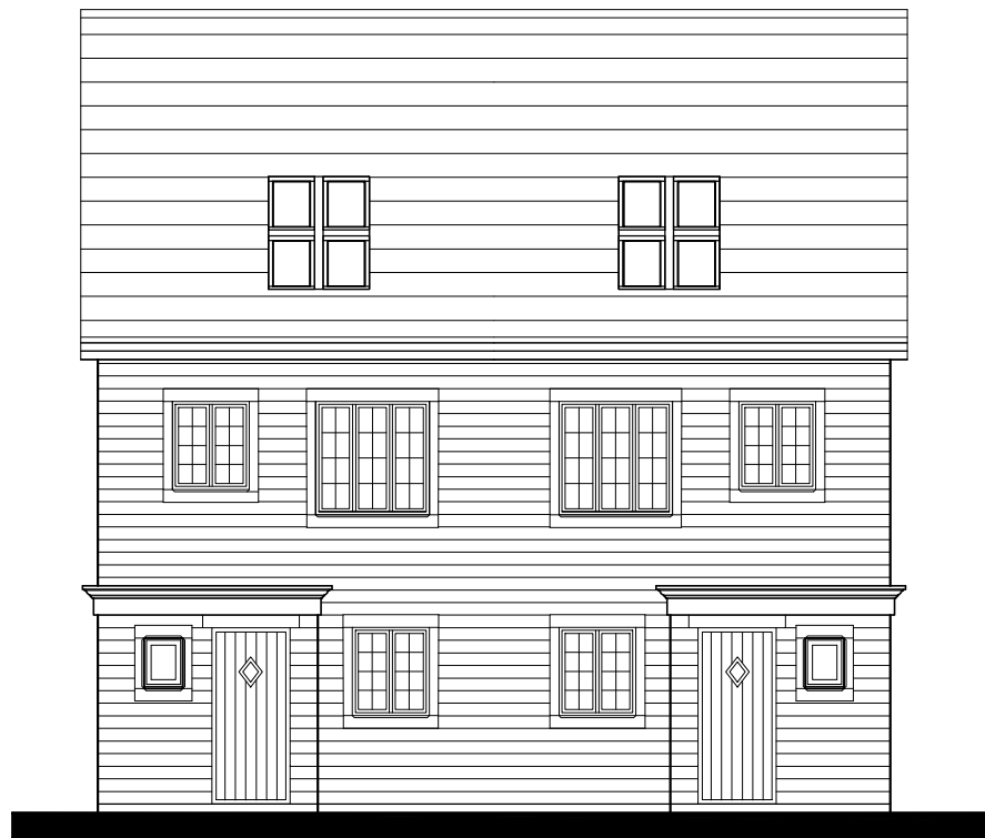
FRONT ELEVATION
