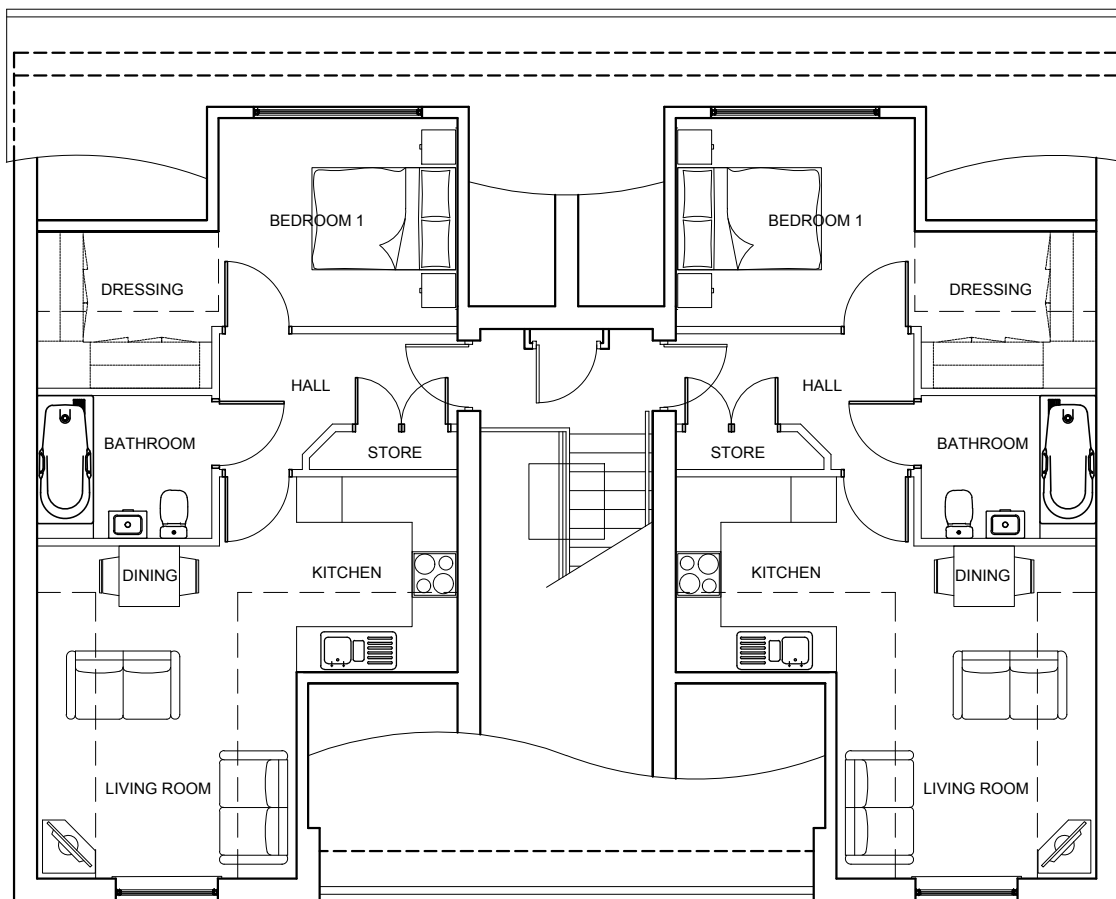
THIRD FLOOR
