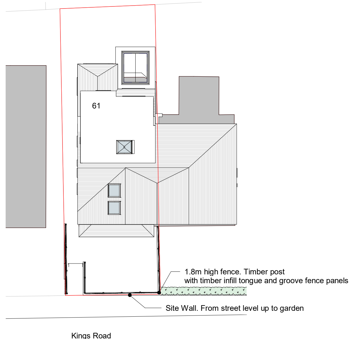
2. Site - Proposed Landscaping Plan 1 : 200
