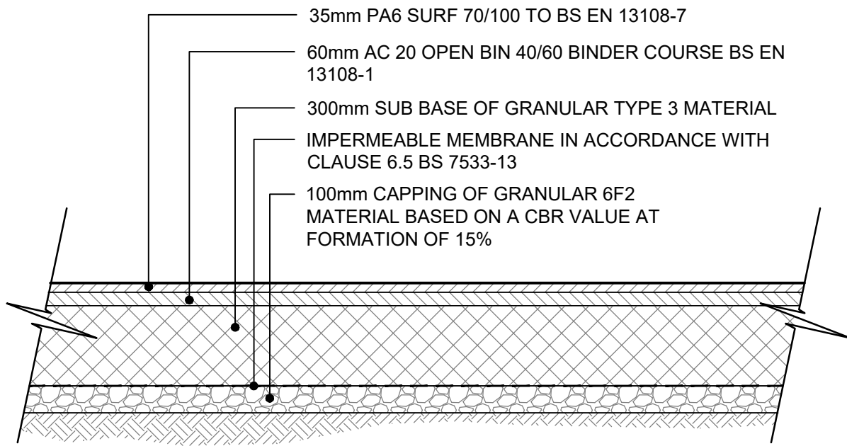
DETAIL 2 PERMEABLE ASPHALT CAR PARK CONSTRUCTION (SCALE 1:20)
