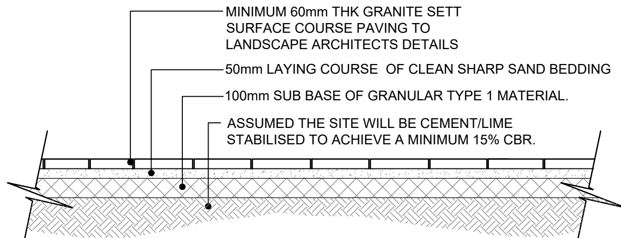
DETAIL 5 GRANITE SETTS PAVING CONSTRUCTION (PEDESTRIAN ACCESS) (SCALE 1:20)
