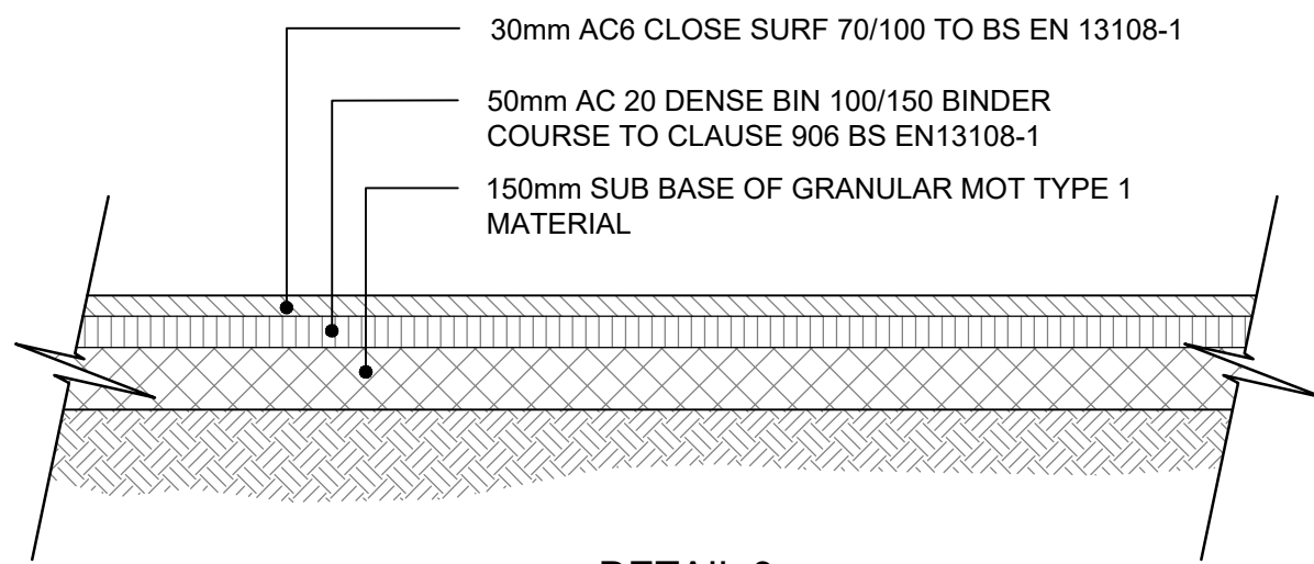
DETAIL 3 ASPHALT FOOTPATH CONSTRUCTION (SCALE 1:20)
