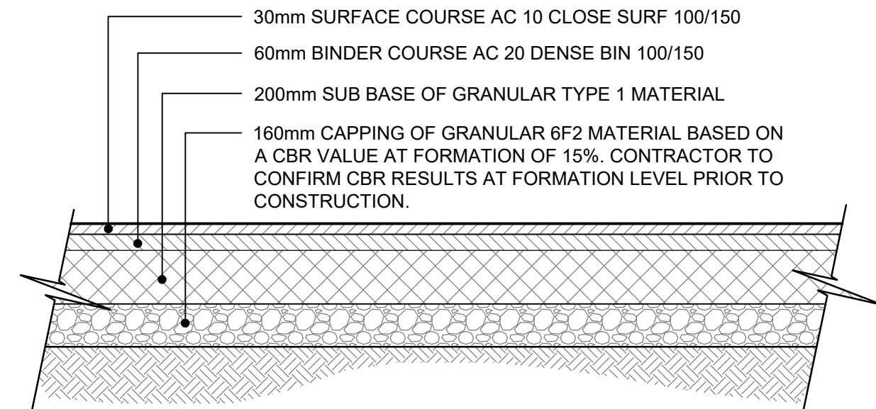
DETAIL 4 ASPHALT CAR PARK CONSTRUCTION (NO HGV ACCESS) (SCALE 1:20)
