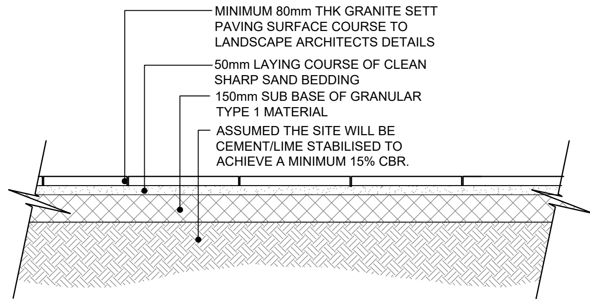
DETAIL 6 GRANITE SETTS PAVING CONSTRUCTION (MEWP ACCESS) (SCALE 1:20)
