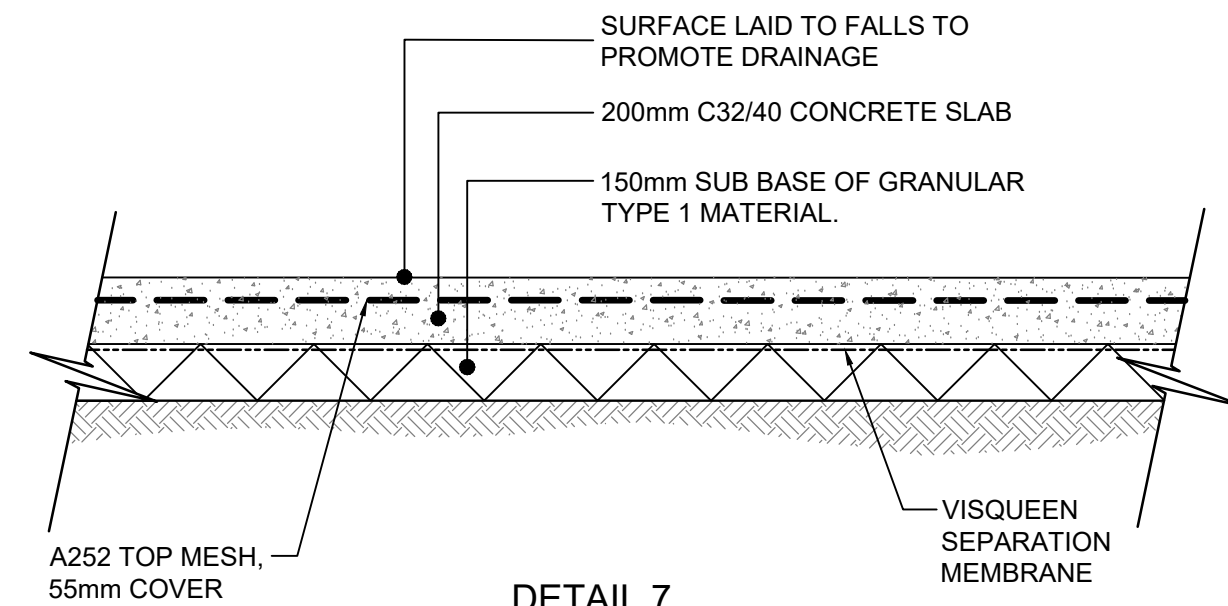
DETAIL 7 INDICATIVE REINFORCED CONCRETE SLAB (SCALE 1:20)
