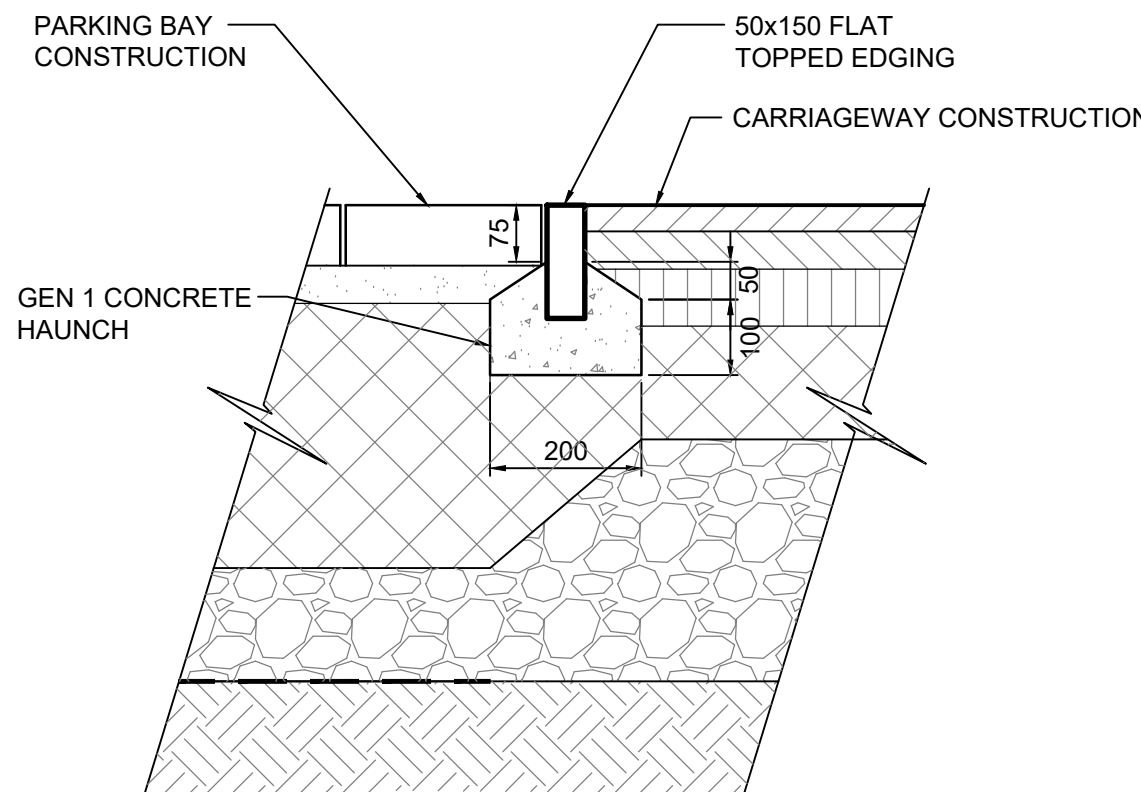
DETAIL 10 EF EDGING KERB (SCALE 1:10)
