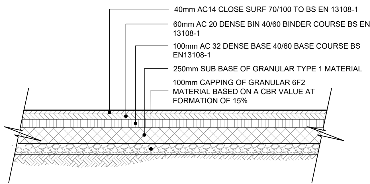
DETAIL 1 ASPHALT CARRIAGEWAY CONSTRUCTION (SCALE 1:20)
