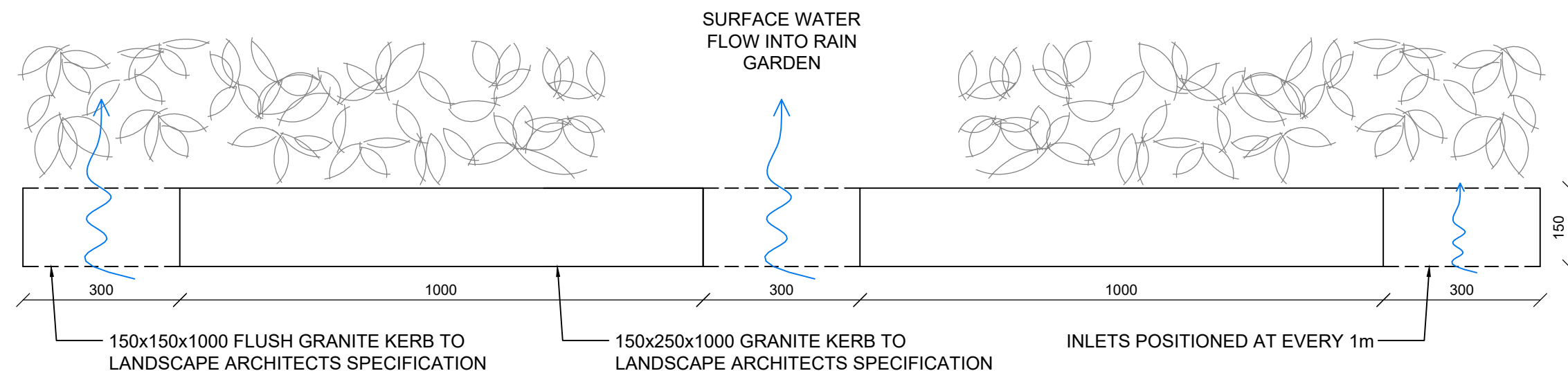
GRANITE RAIN GARDEN GRANITE KERB - PLAN (SCALE 1:10)
