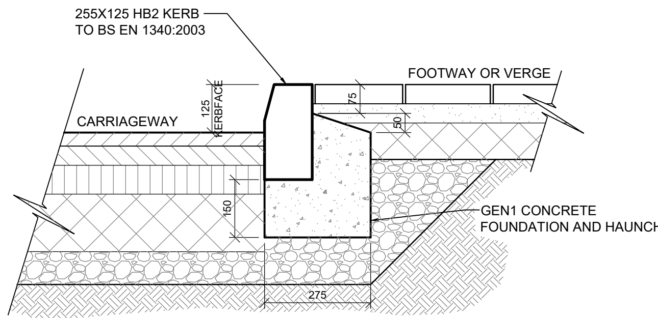
DETAIL 9 HB2 ROAD KERB (SCALE 1:10)
