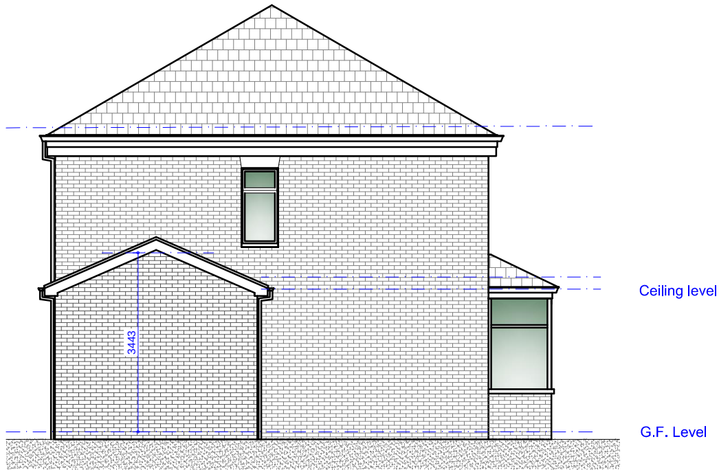
Existing L/H Side Elevation Scale 1:100
