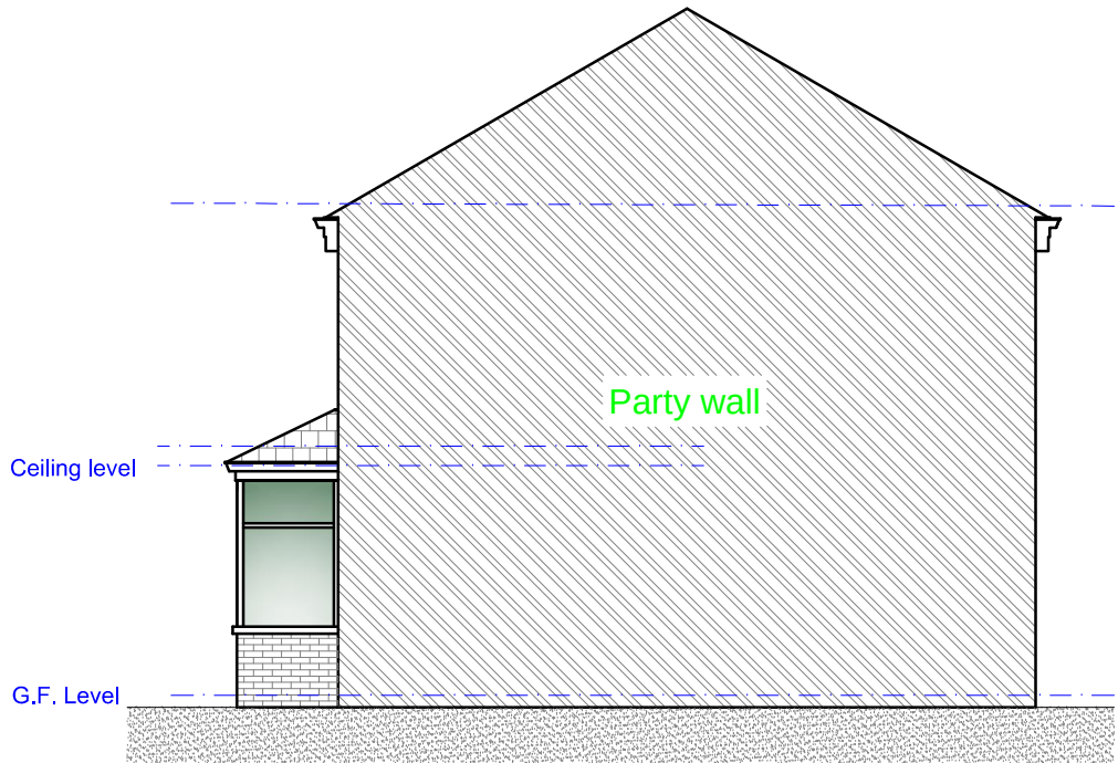
Existing R/H Side Party Wall Elevation Scale 1:100
