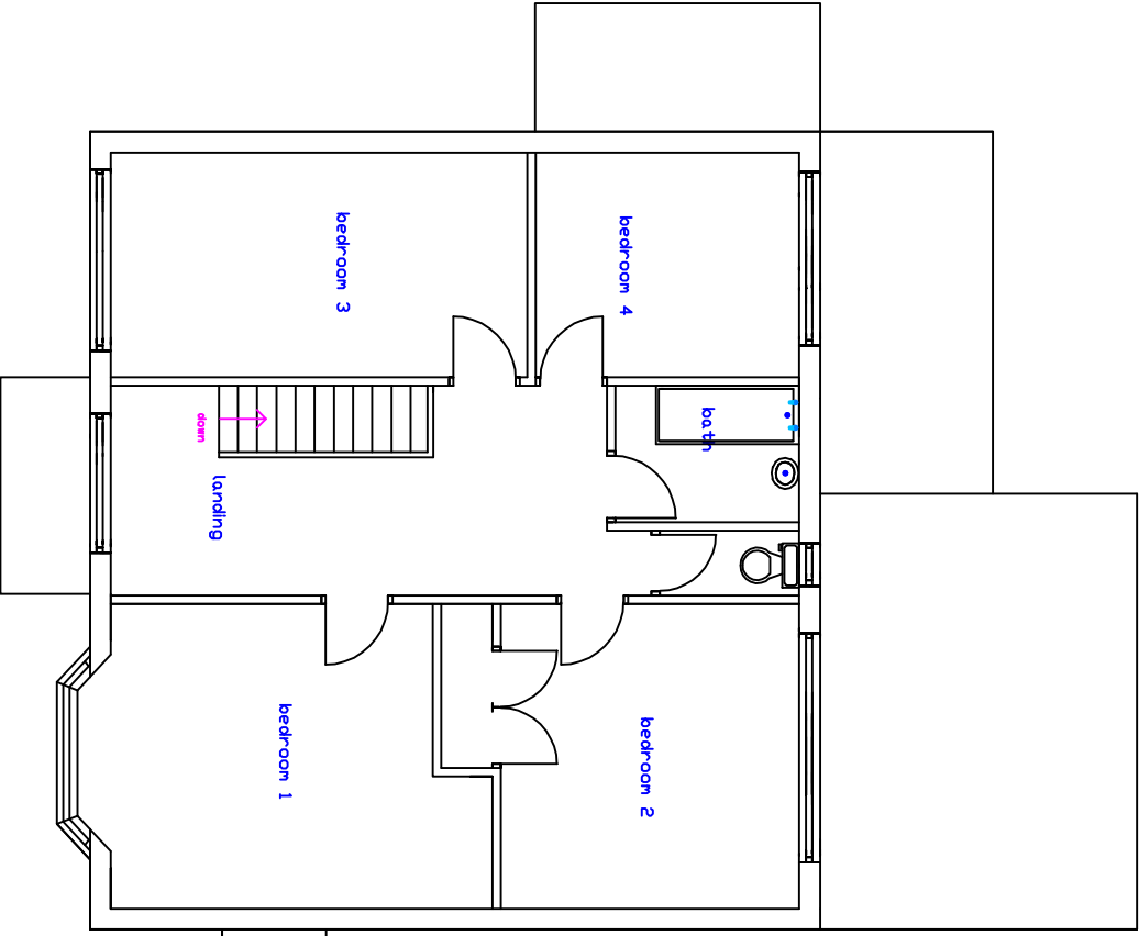
FORMER FIRST FLOOR LAYOUT 1:100
