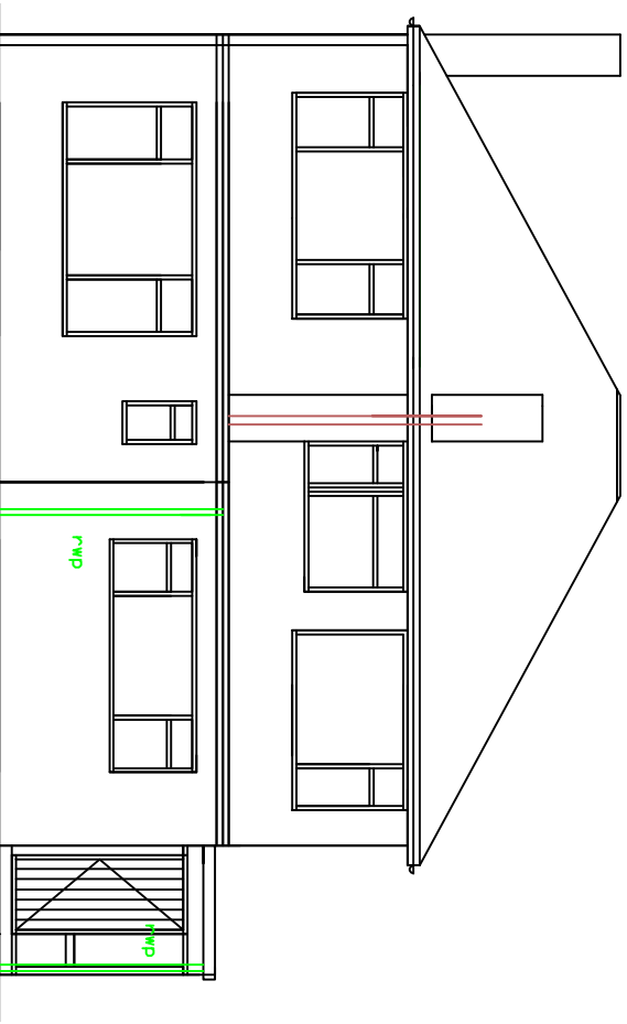
FORMER REAR VIEW 1:100
