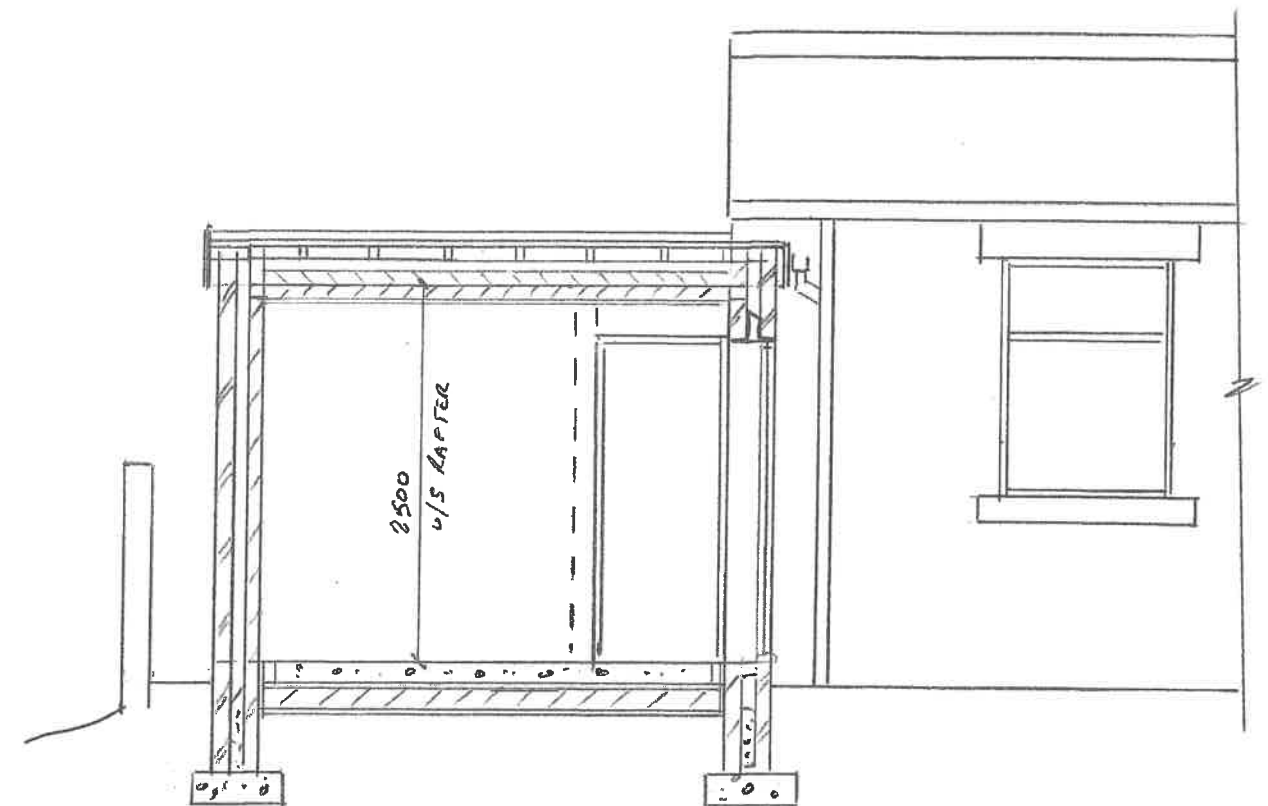
SECTION THROUGH
